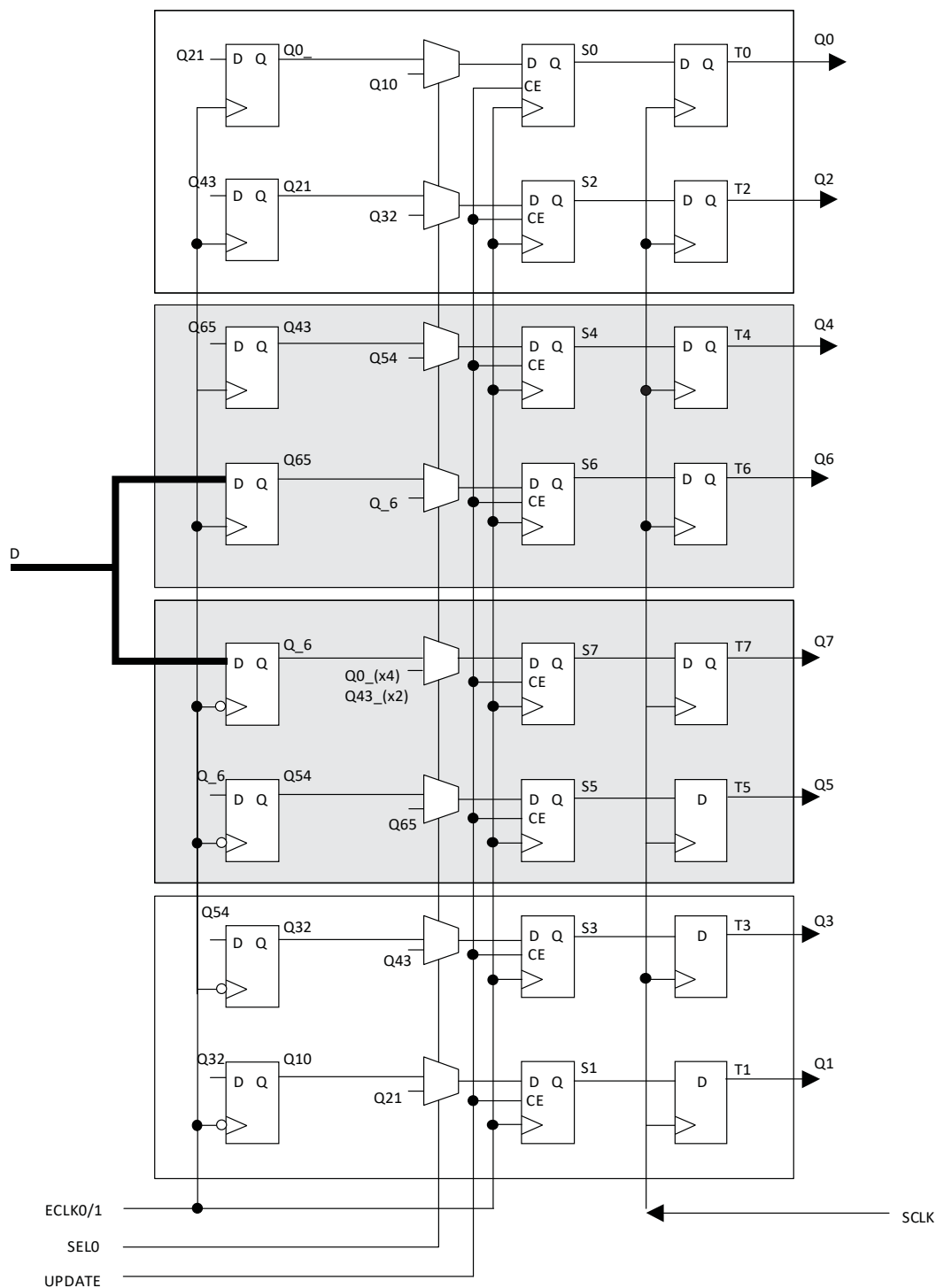
Figure 2.16. Input Gearbox
