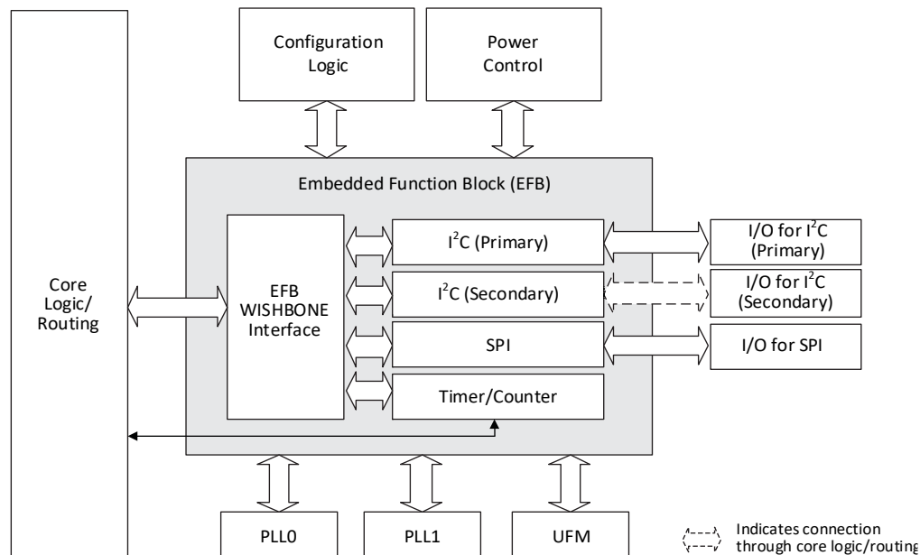
Figure 2.20. MachXO2-256, MachXO2-640/U and MachXO2-1200 Banks
