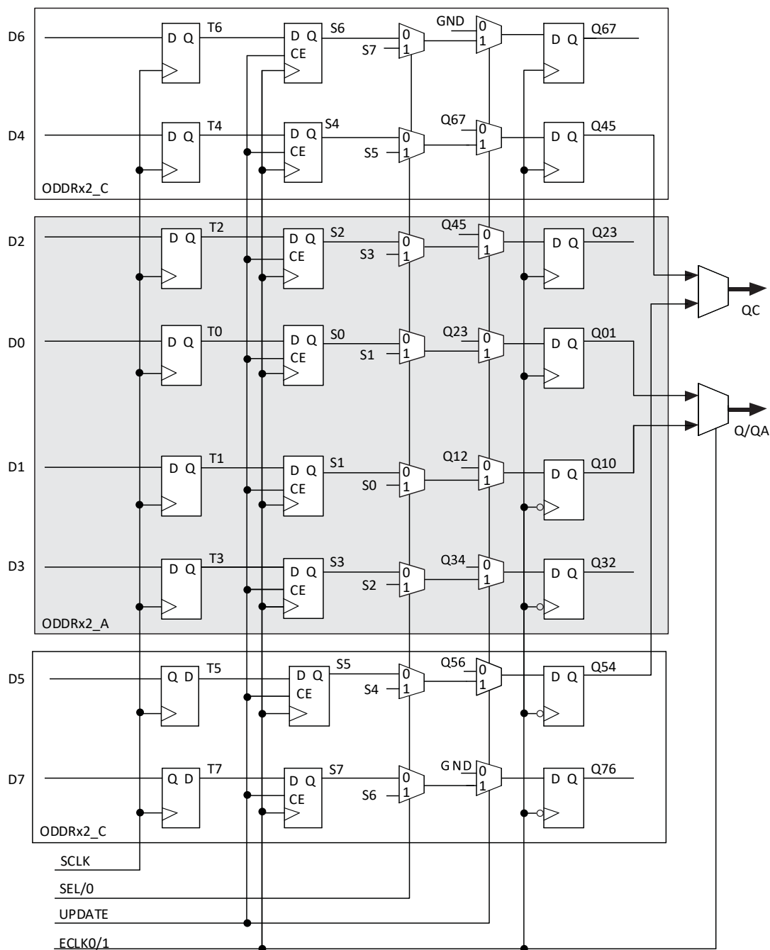
Figure 2.17. Output Gearbox
