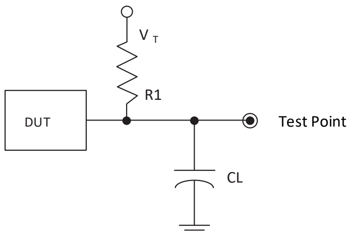
Figure 3.15. Output Test Load, LVTTTL and LVCMOS Standards
