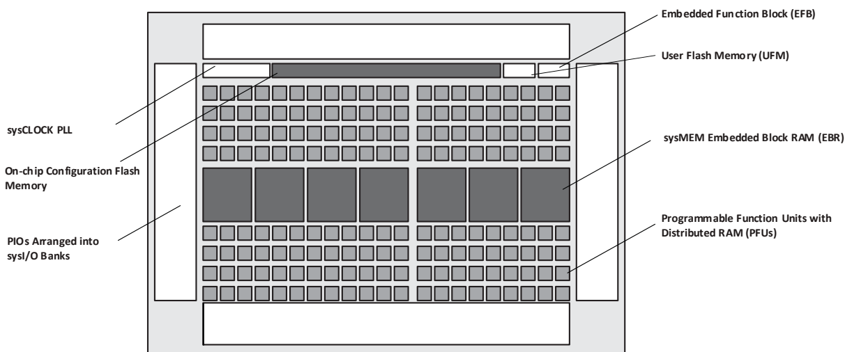
Figure 2.1. Top View of the MachXO2-1200 Device
