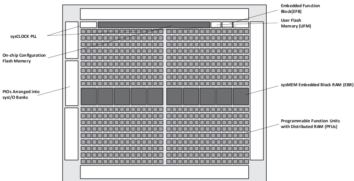
Figure 2.1. Top View of the MachXO2-1200 Device
