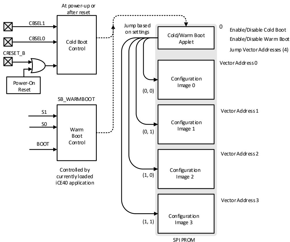
Figure 10.1. Cold Boot and Warm Boot Configuration
