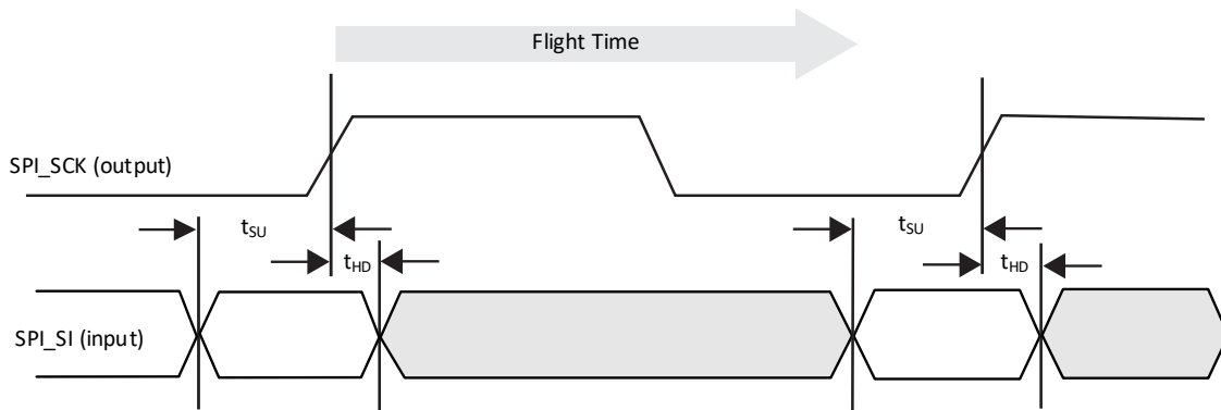
Figure 9.2. SPI Master Configuration Timing
