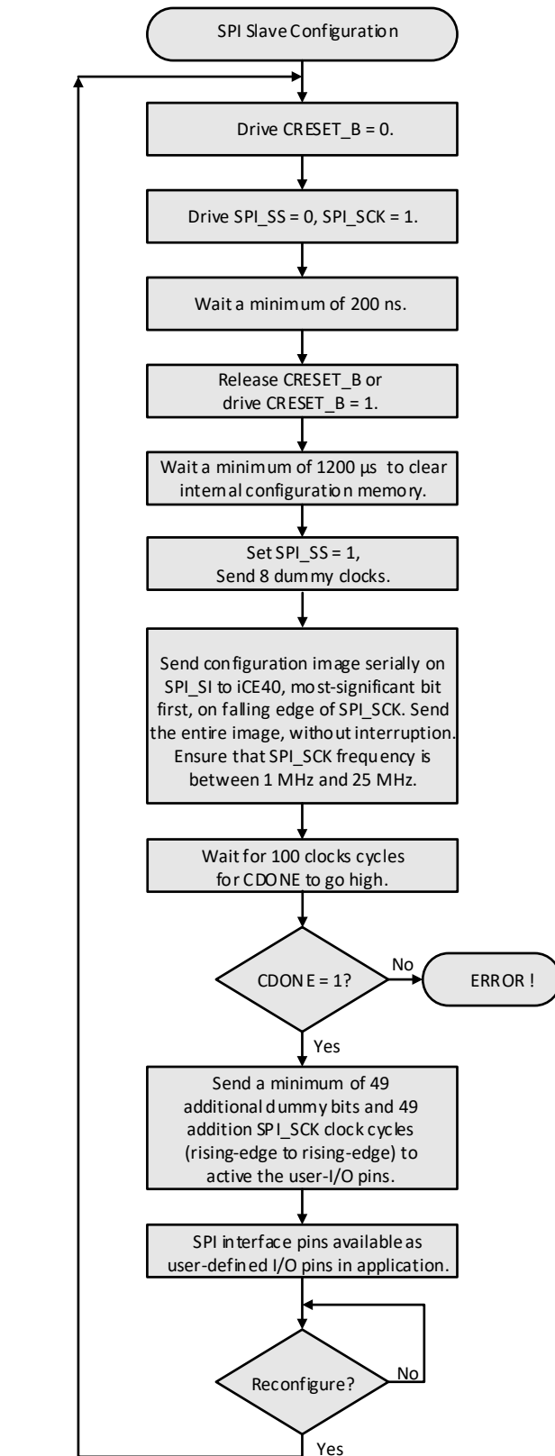
Figure 13.3. SPI Slave Configuration Process
