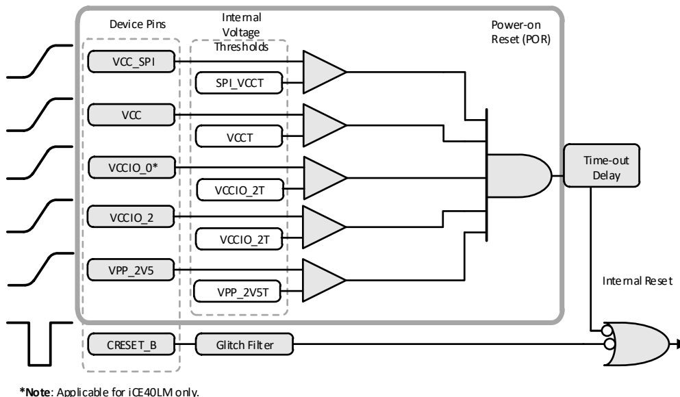
Figure 7.1. iCE40 Internal Reset Circuitry
