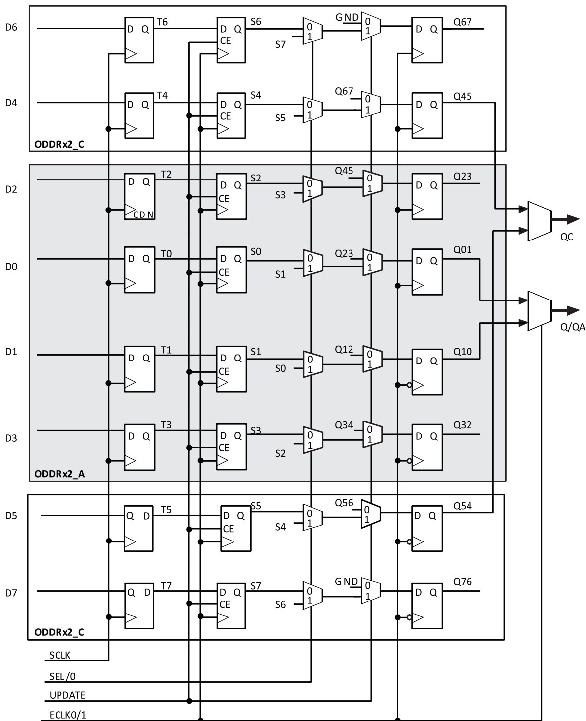
Figure 2.14. Output Gearbox
