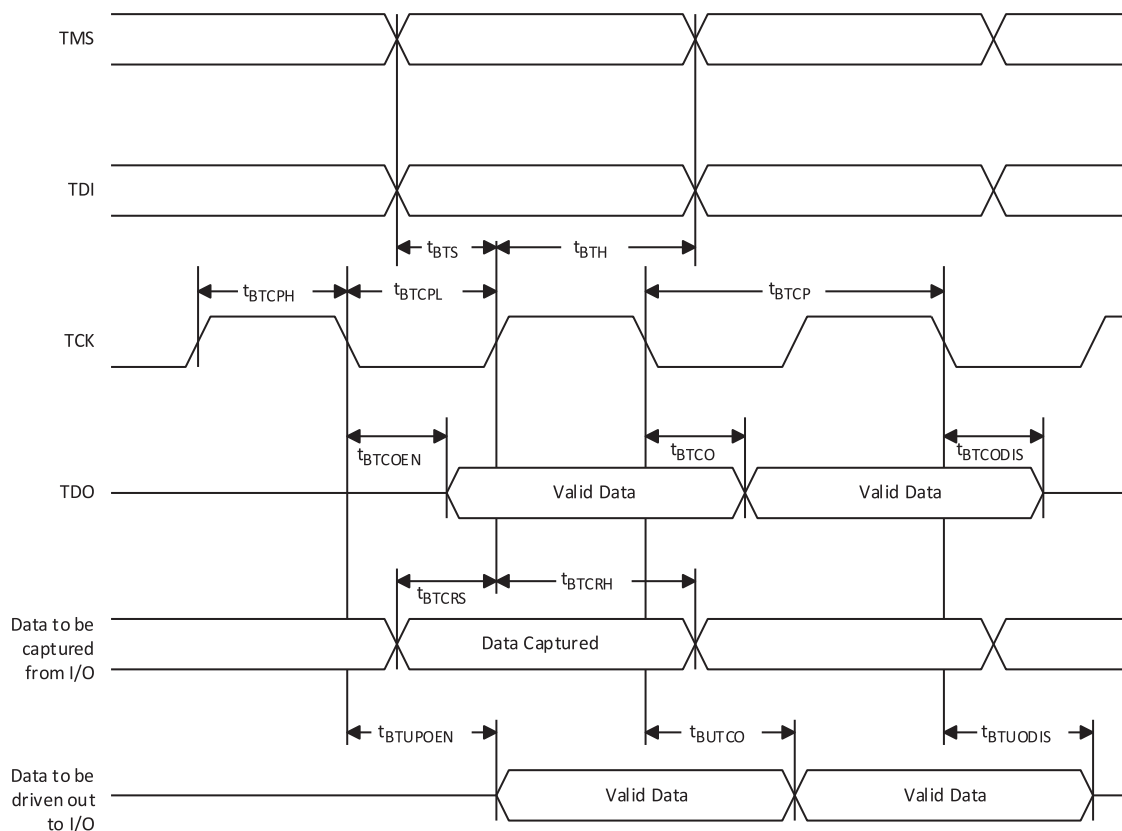
Figure 3.9. JTAG Port Timing Waveforms
