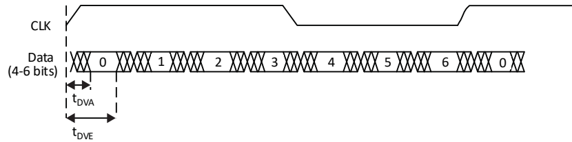
Figure 3.7. Receiver GDDR71_RX. Waveforms
