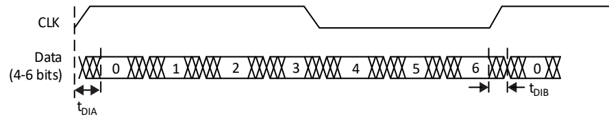
Figure 3.8. Transmitter GDDR71_TX. Waveforms
