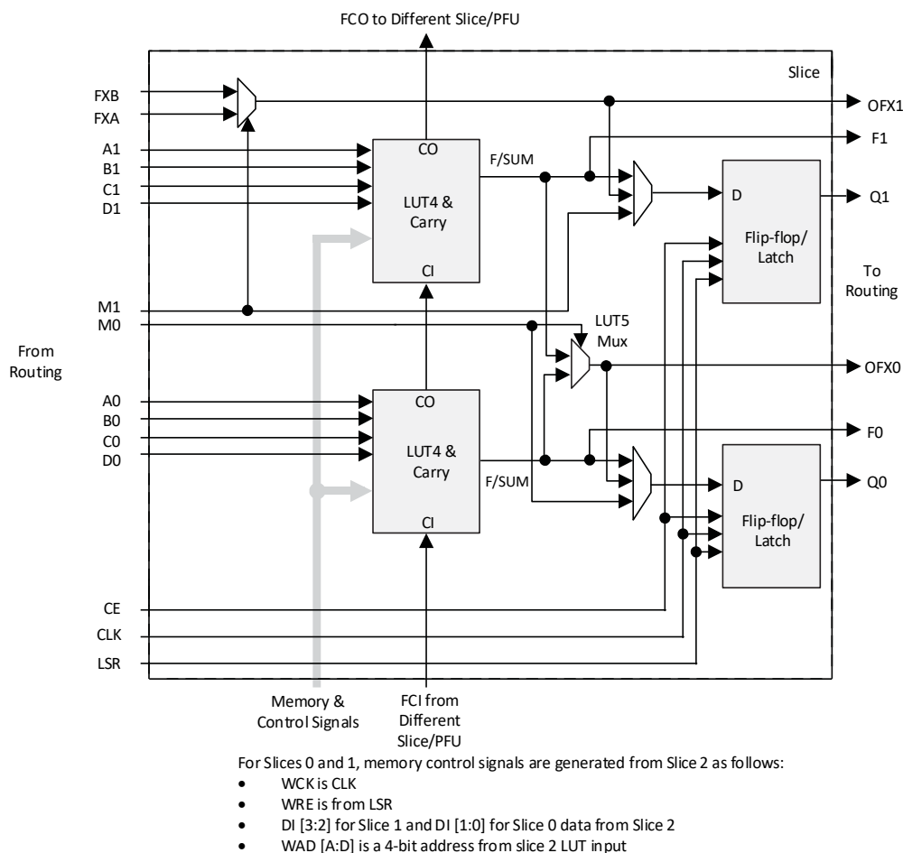
Figure 2.4. Slice Diagram
