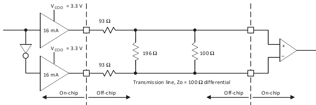
Figure 3.3. Differential LVPECL
