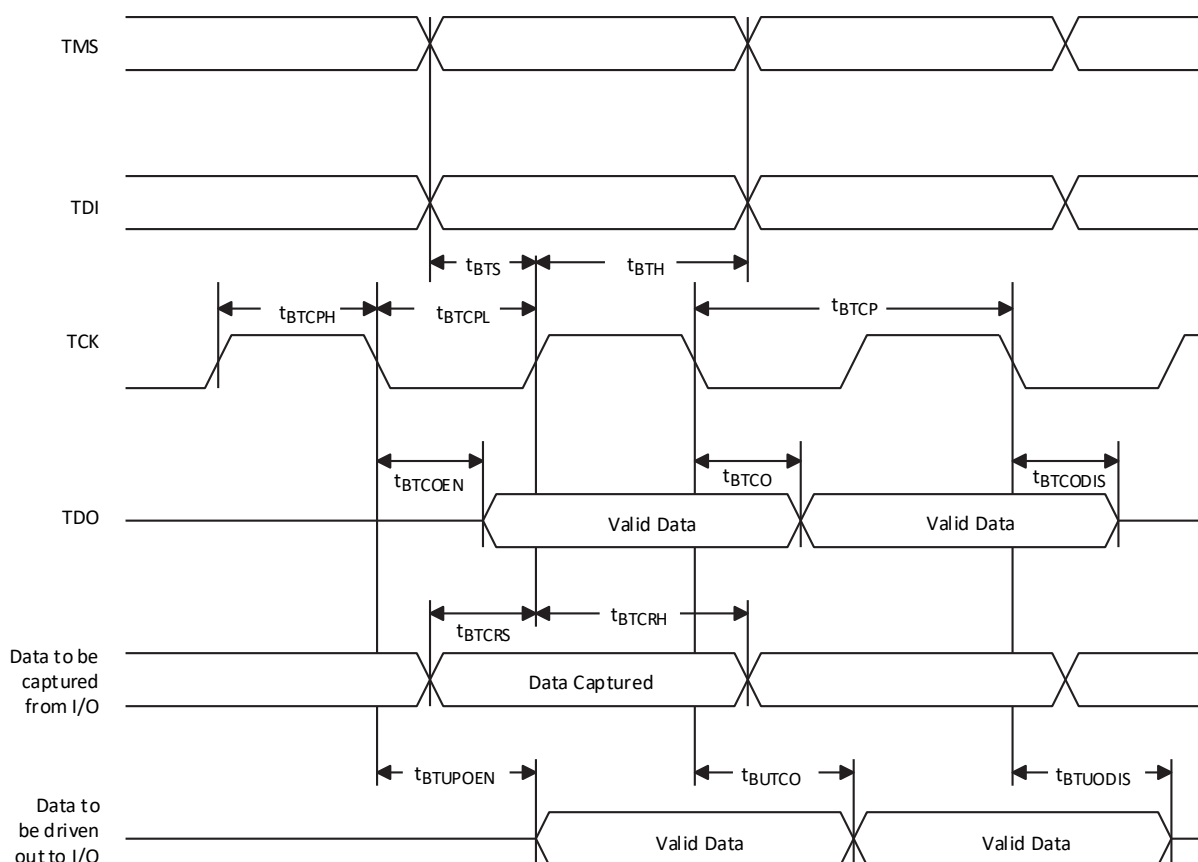
Figure 3.9. JTAG Port Timing Waveforms
