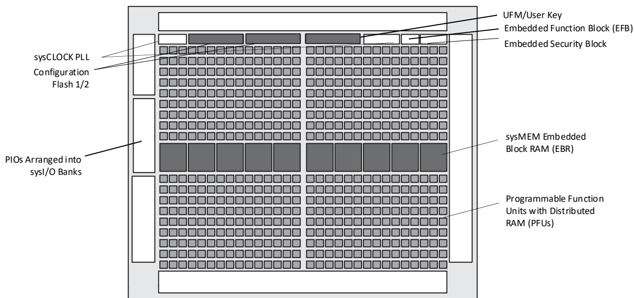
Figure 2.1. Top View of the MachXO3D Device
