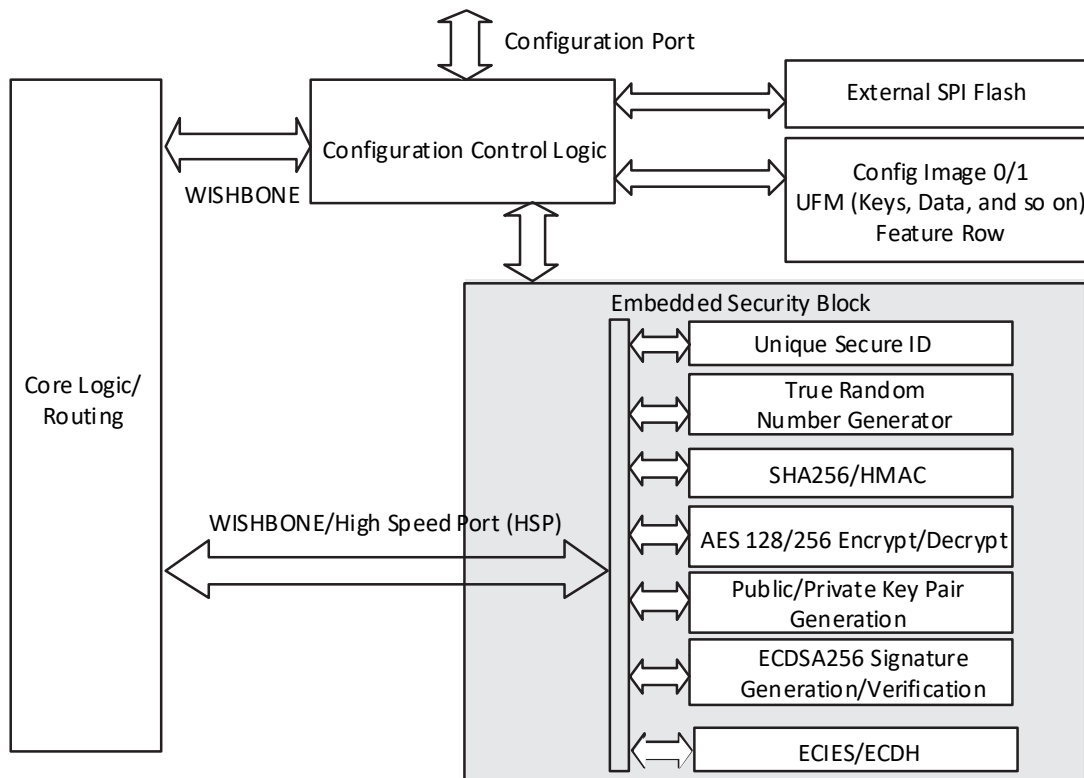
Figure 2.16. ESB Core Block Diagram
