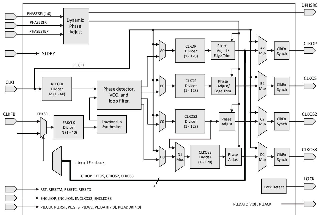
Figure 2.6. PLL Diagram
