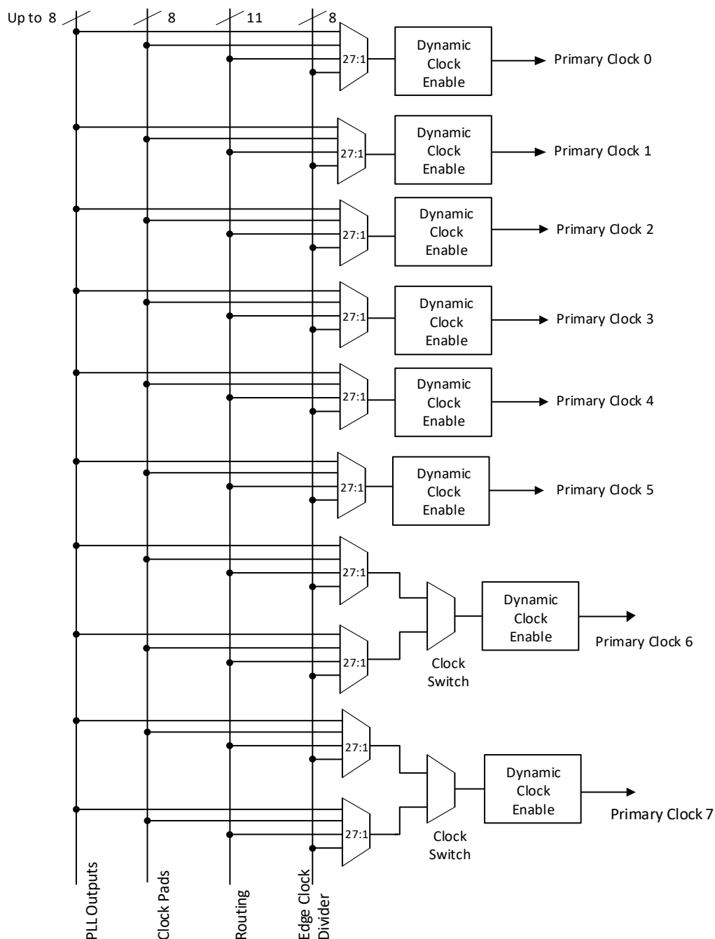
Figure 2.4. Primary Clocks for MachXO3D Devices
