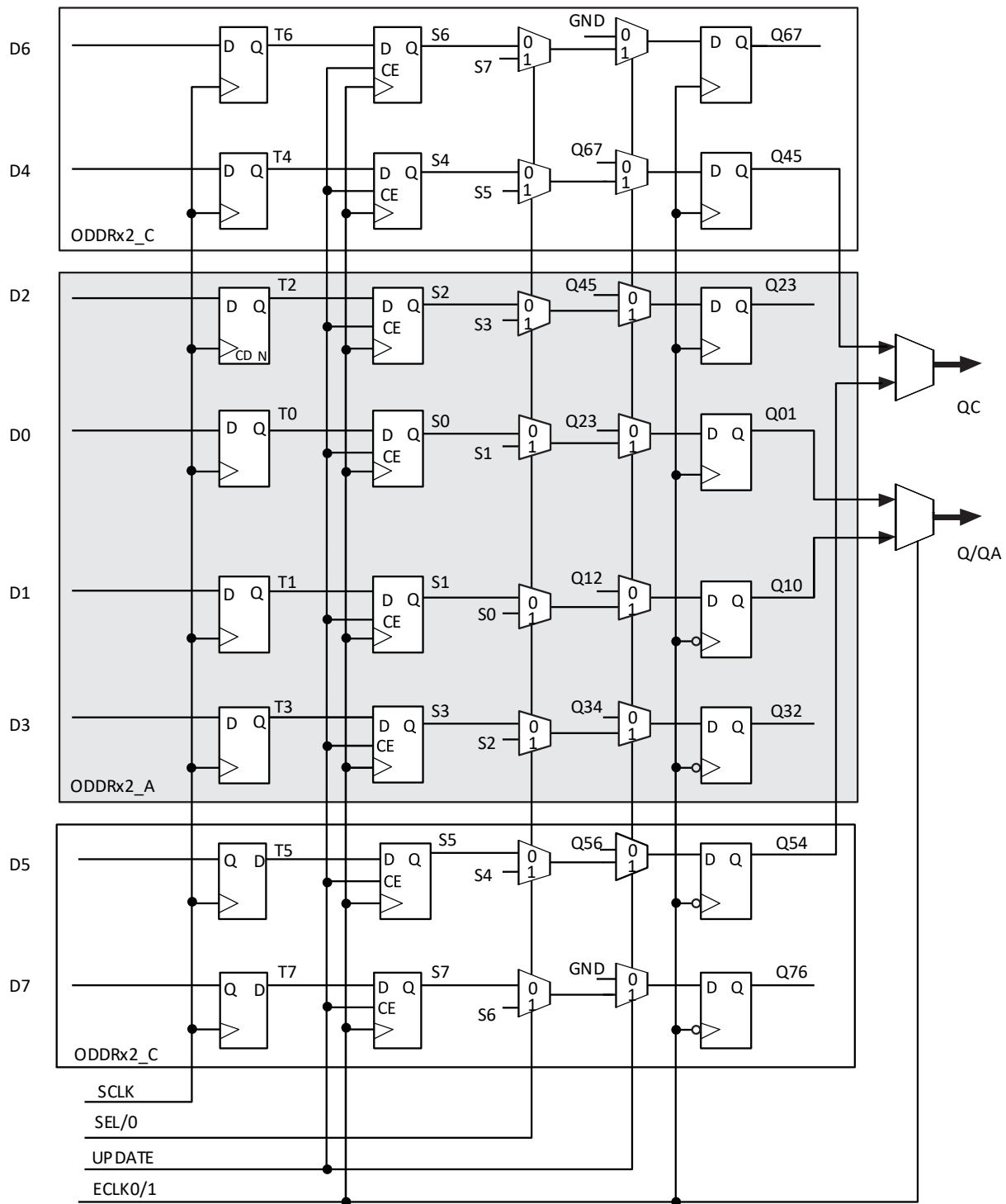
Figure 2.13. Output Gearbox
