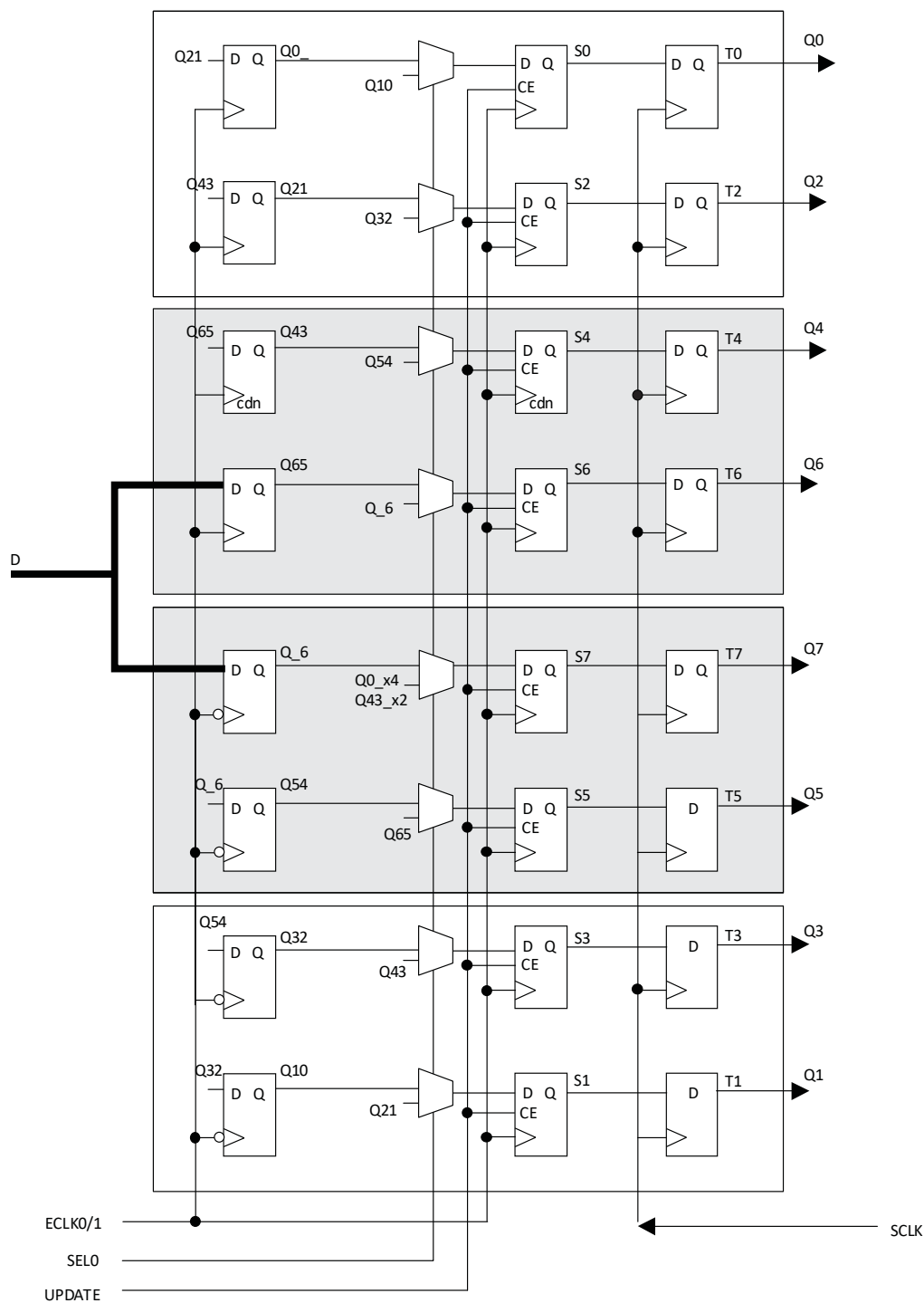
Figure 2.12. Input Gearbox
