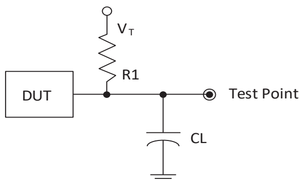
Figure 3.10. Output Test Load, LVTTTL and LVCMOS Standards
