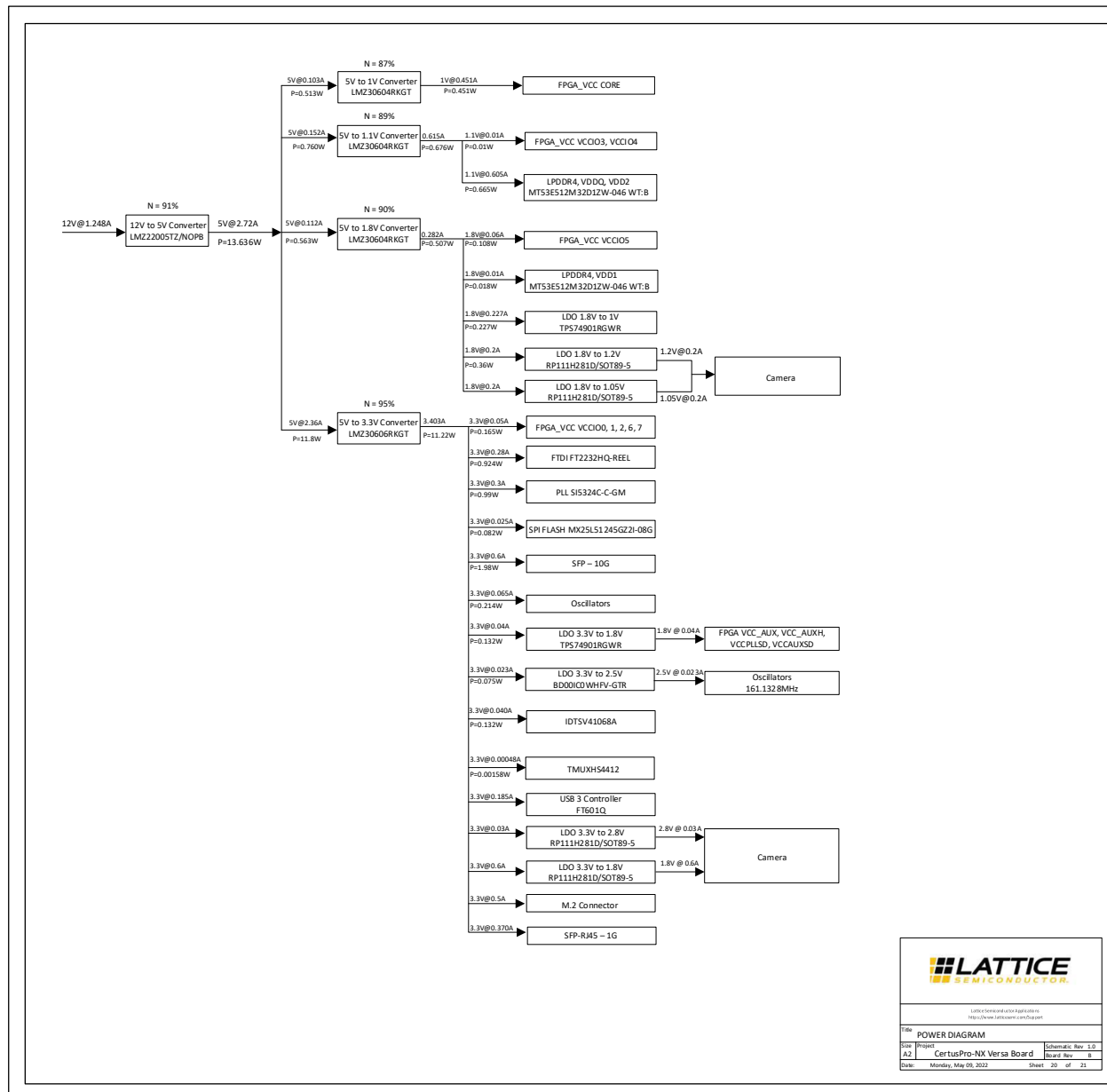
Figure A.20. POWER DIAGRAM
