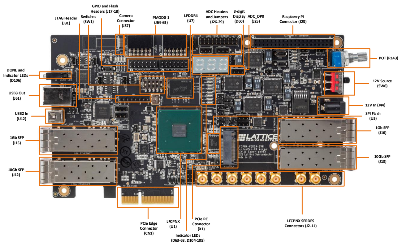
Figure 1.1. Top View of CertusPro-NX Versa Evaluation Board
