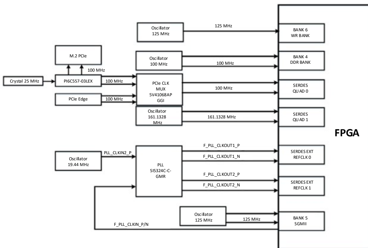
Figure 4.1. Clock Scheme
