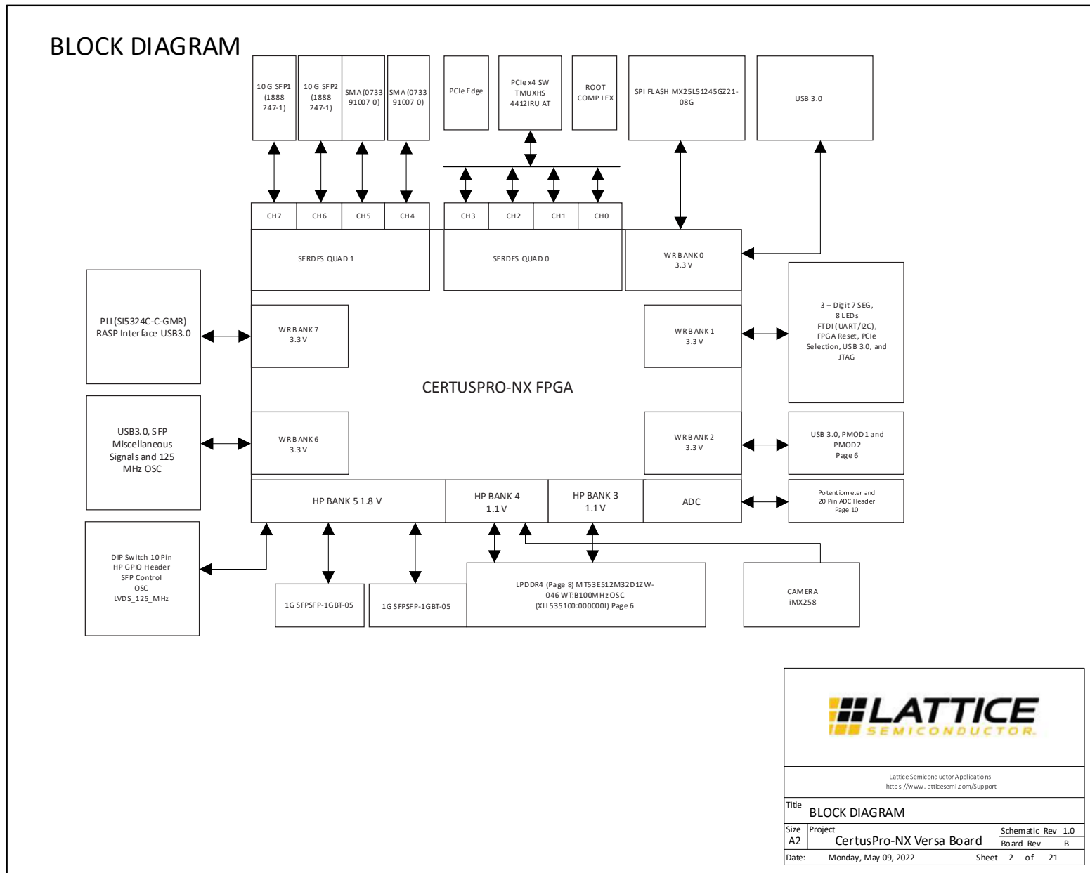
Figure A.2. Block Diagram
