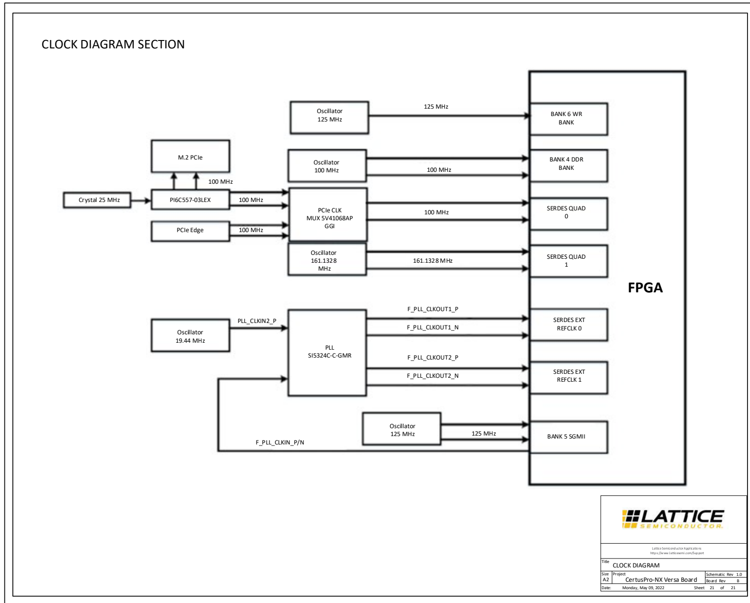
Figure A.21. CLOCK DIAGRAM
