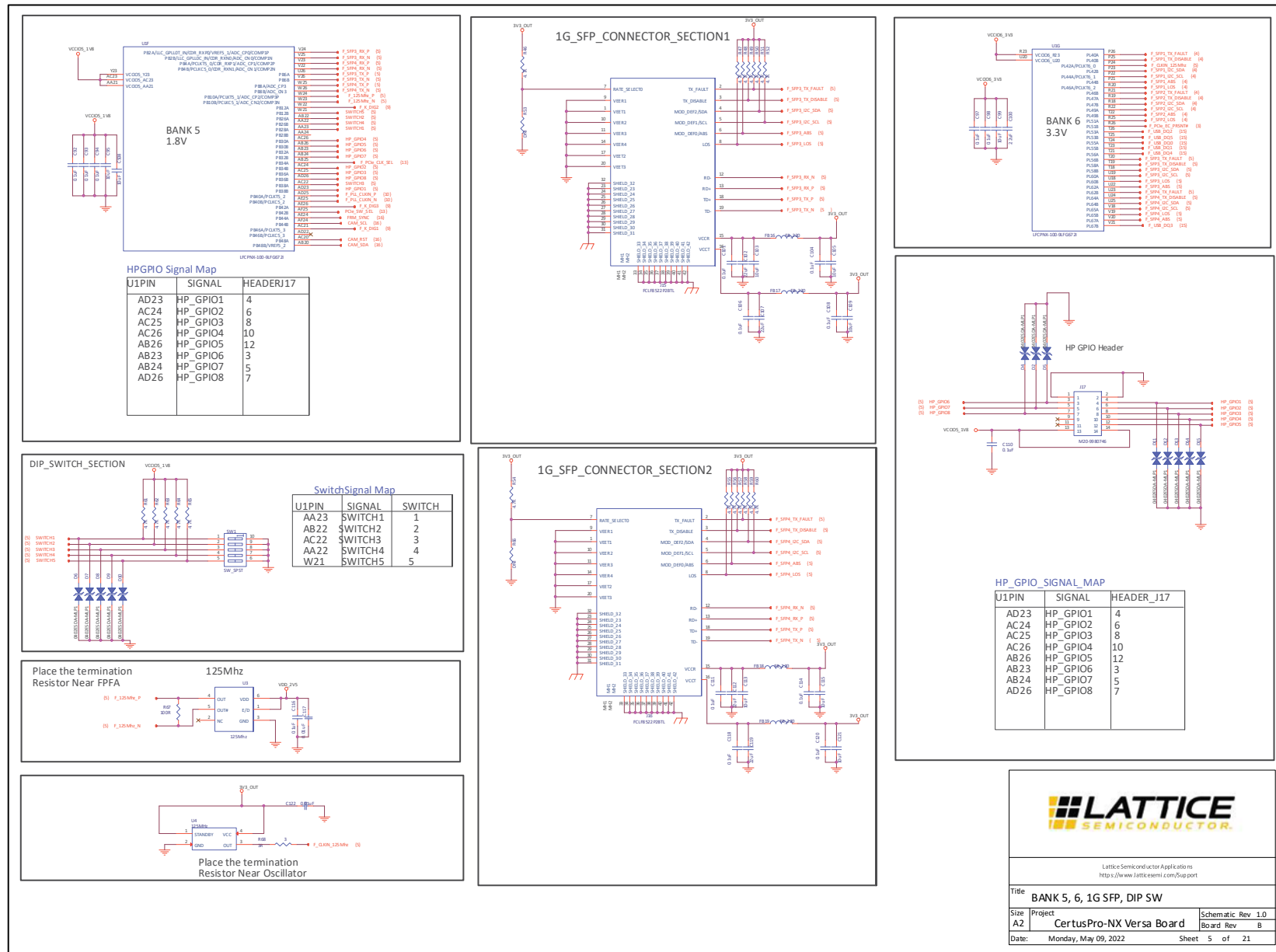
Figure A.5. Bank 5 and 6, 1G SFP DIP SW, HP GPIO HEADER
