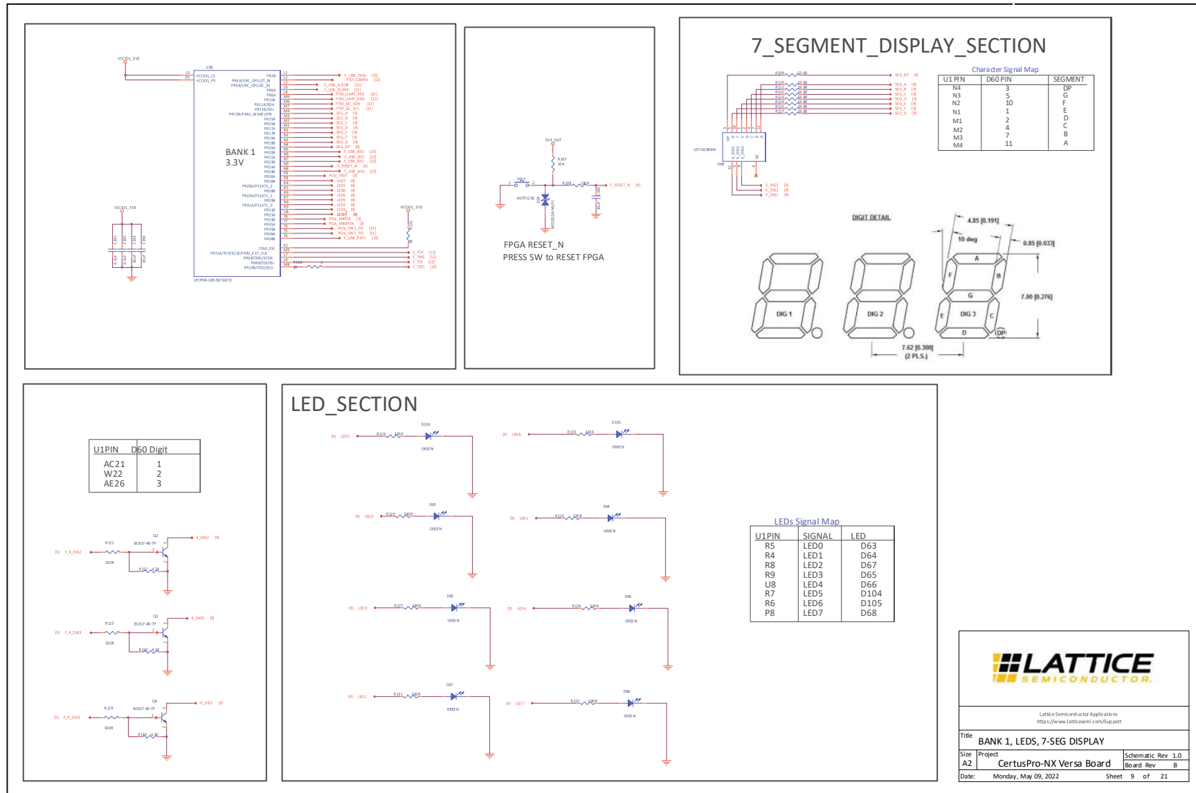
Figure A.9. BANK 1, LEDS, 7 SEGMENT DISPLAY
