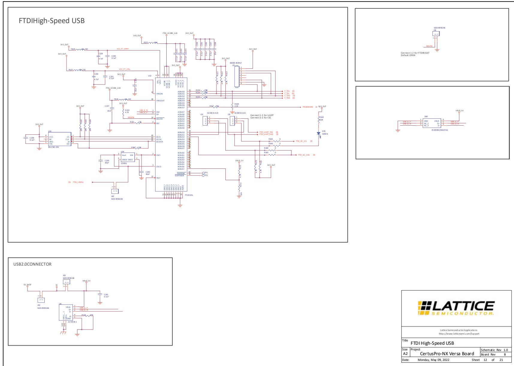
Figure A.12. FTDI High-speed USB
