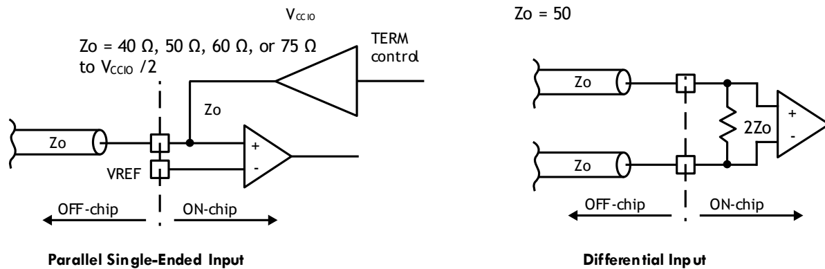
Figure 4.1. On-Chip Termination
