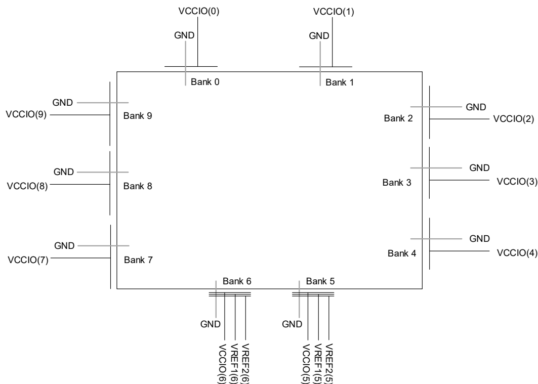
Figure 2.32. sysI/O Banking of MachXO5-NX-25 Devices
