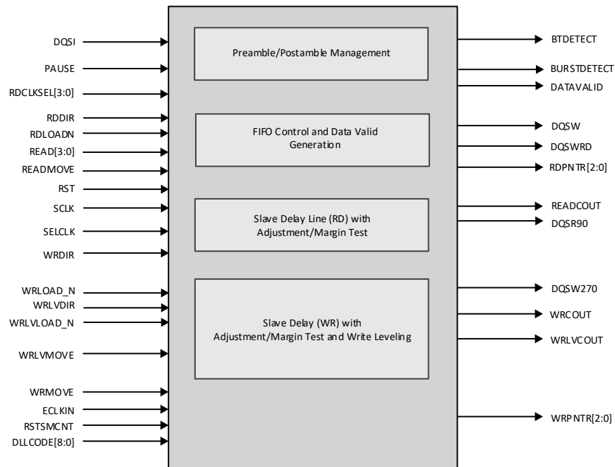
Figure 2.31. DQS Control and Delay Block (DQSBUF)
