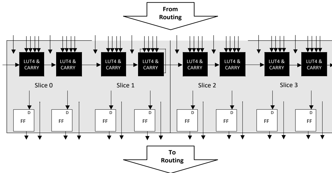
Figure 2.5. PFU Diagram
