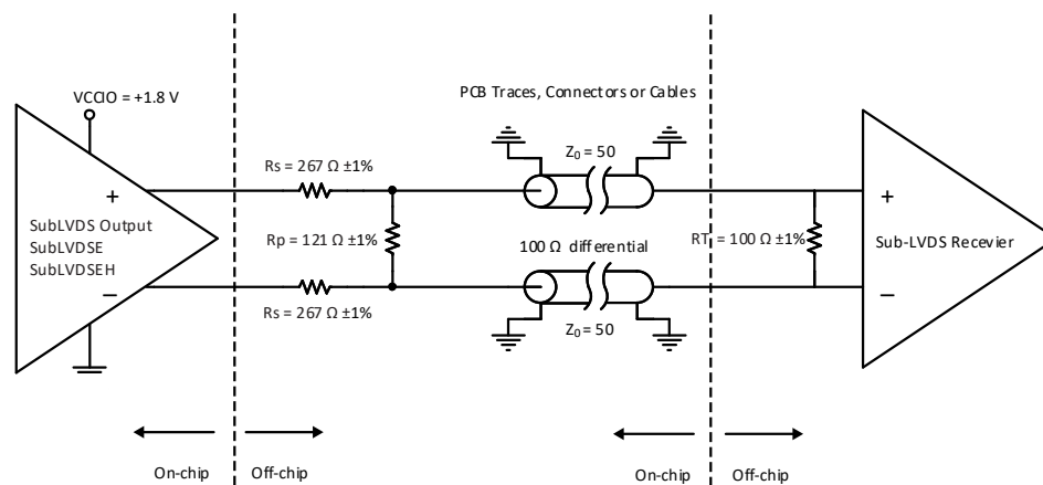
Figure 3.4. SubLVDS Output Interface
