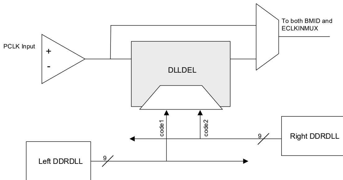
Figure 2.15. DLLDEL Functional Diagram
