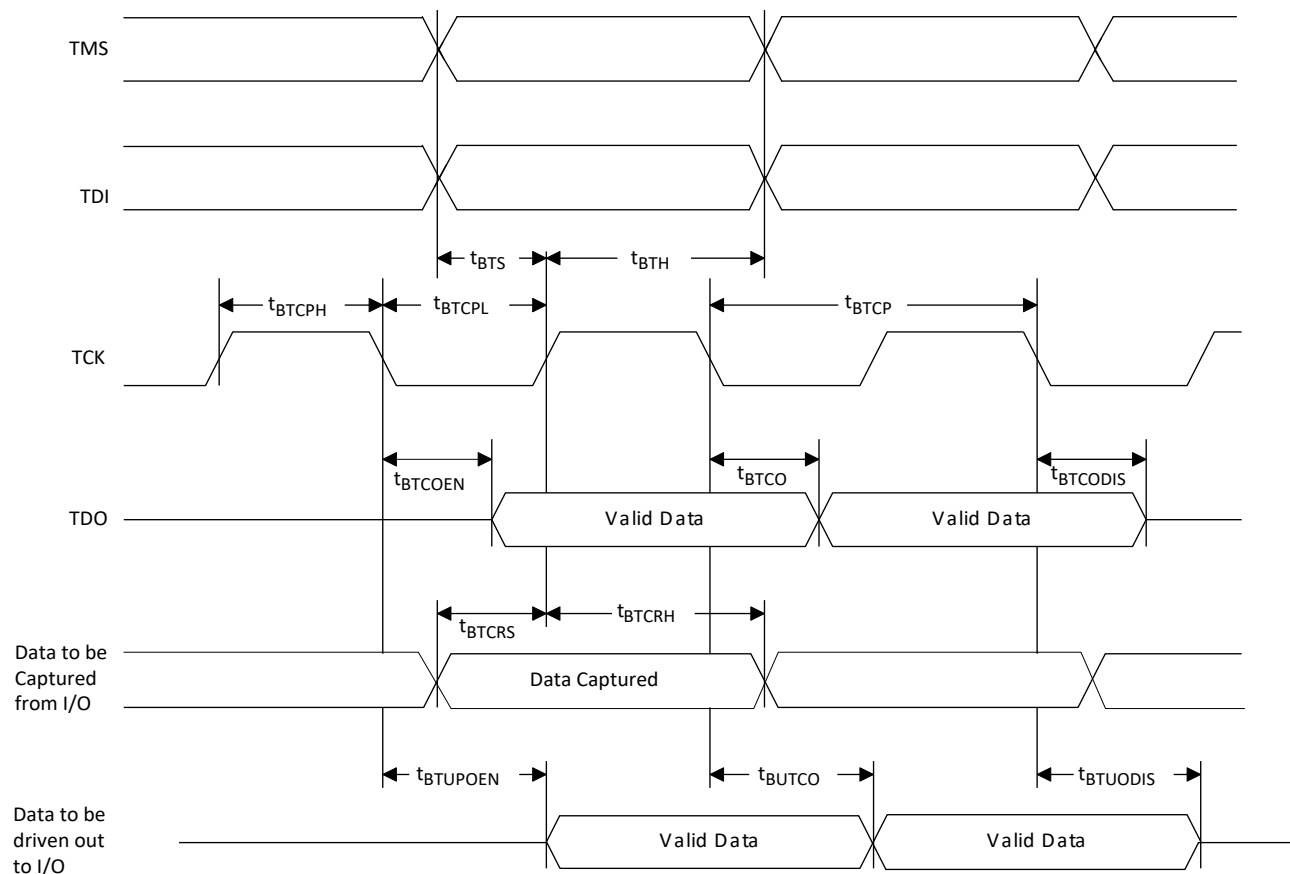
Figure 3.20. JTAG Port Timing Waveforms
