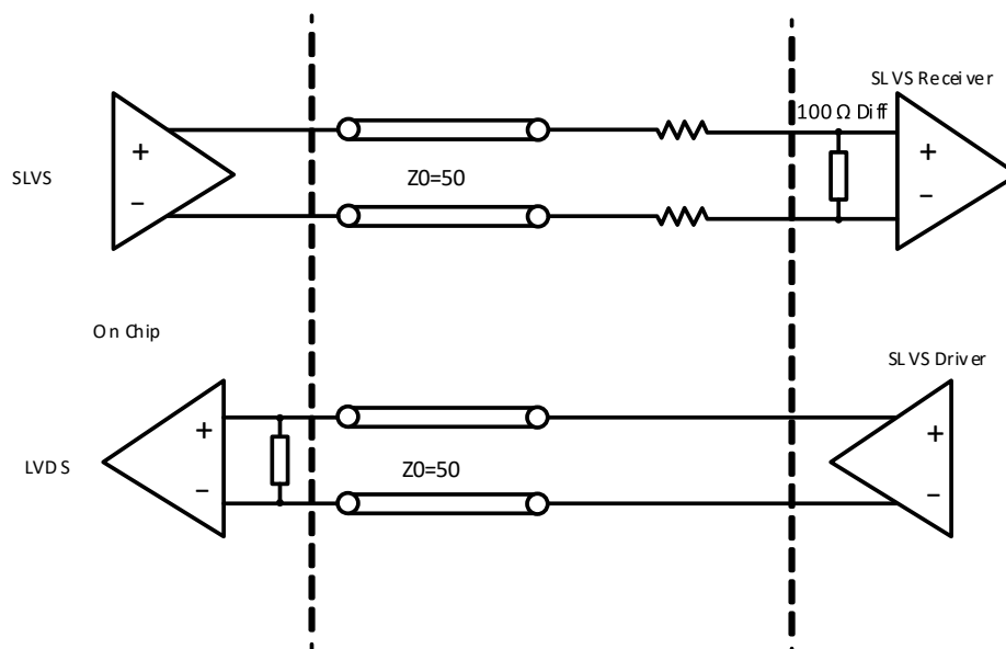
Figure 4.5. SLVS Interface
