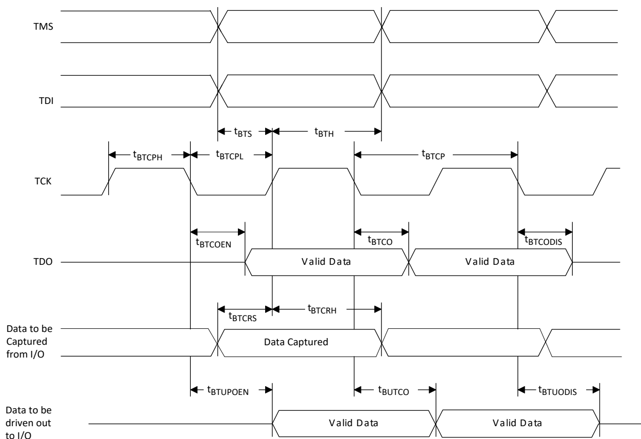
Figure 4.20. JTAG Port Timing Waveforms
