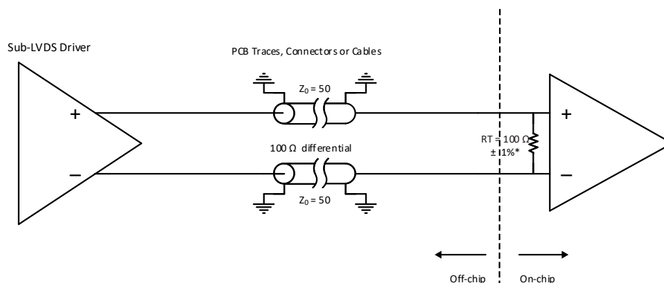
Figure 4.3. SubLVDS Input Interface
