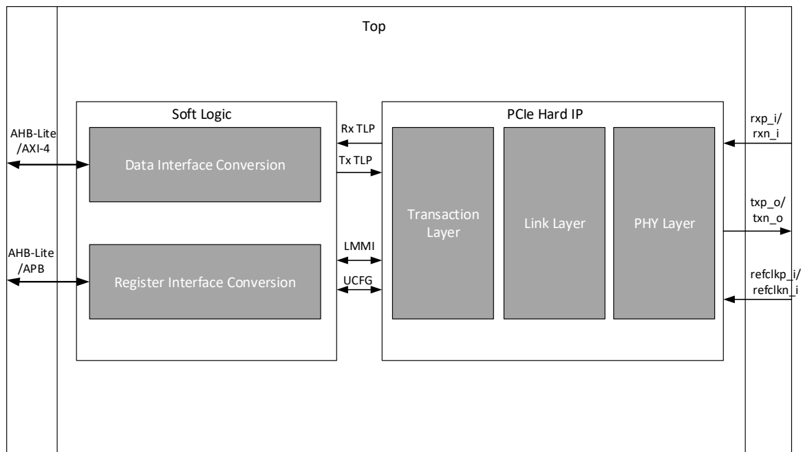
Figure 2.36. PCIe Soft IP Wrapper
