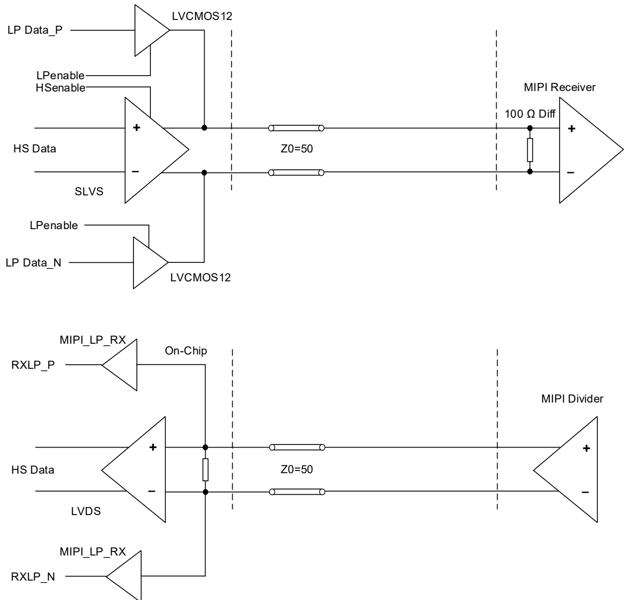
Figure 4.6. MIPI Interface
