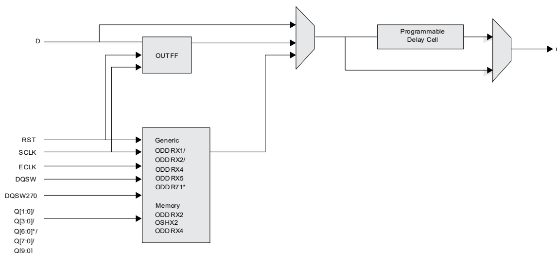
Figure 2.27. Output Register Block on Bottom Side
