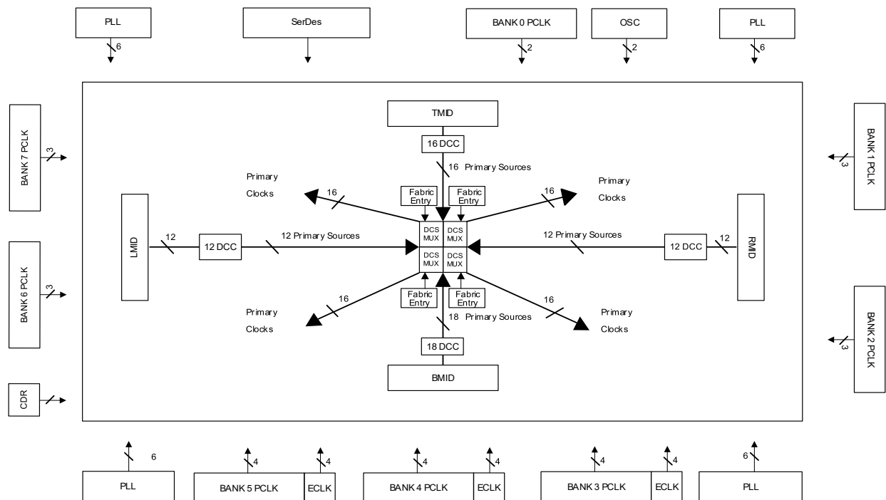
Figure 2.10. Clocking for MachXO5-NX-55T/MachXO5-NX-100T Devices
