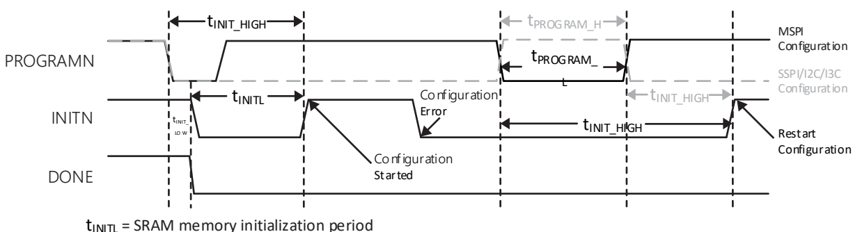
Figure 4.14. Configuration Error Notification (2)
