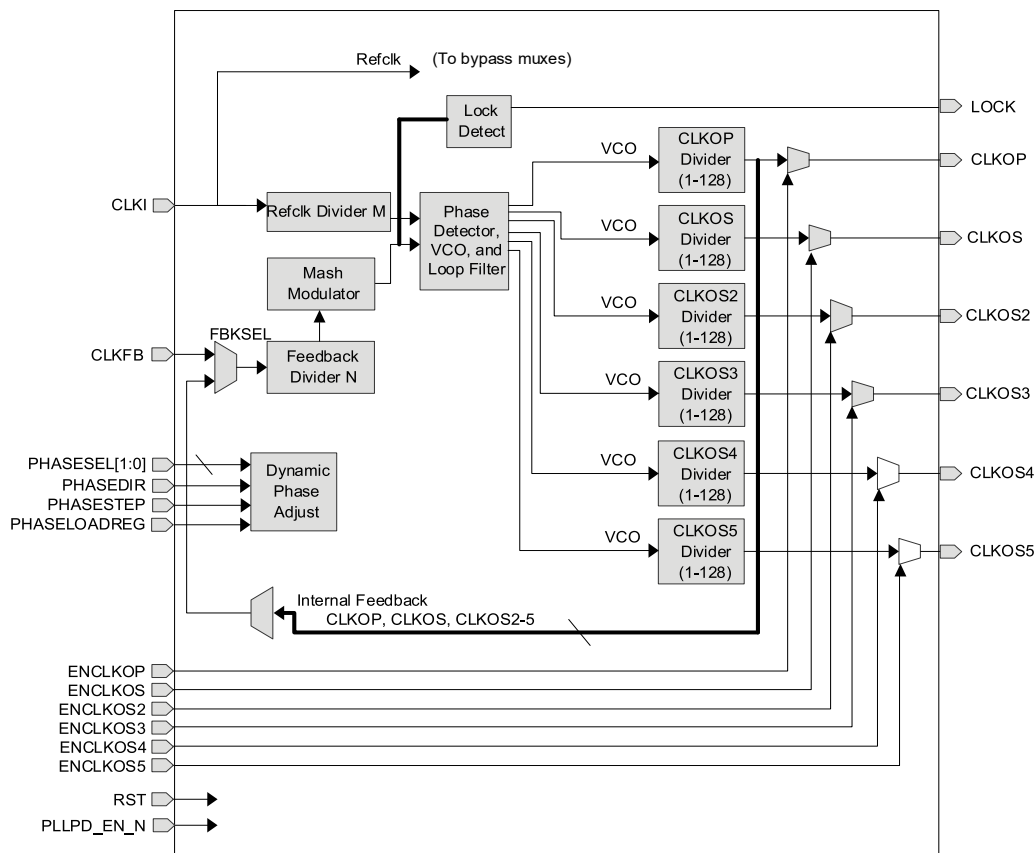
Figure 2.8. General Purpose PLL Diagram
