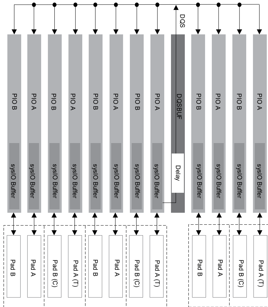
Figure 2.30. DQS Grouping on the Bottom Edge
