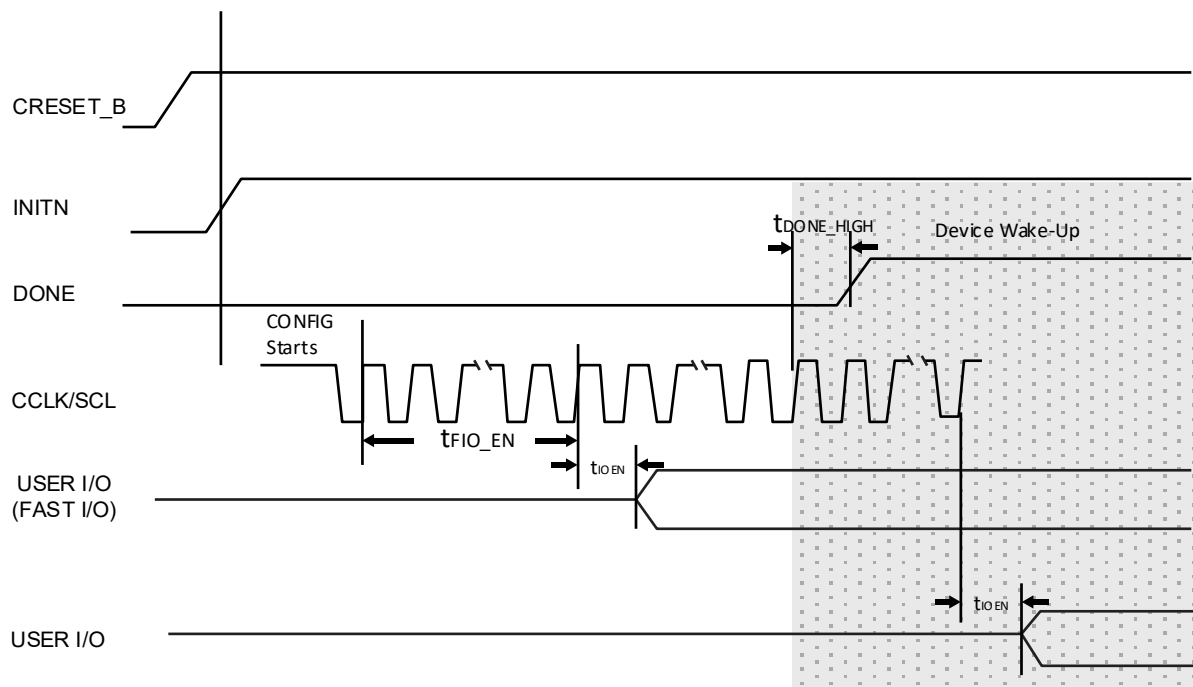
Figure 3.19. Slave SPI/I2C/I3C Wake-Up Timing
