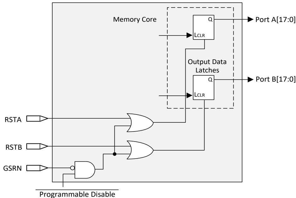
Figure 2.19. Memory Core Reset
