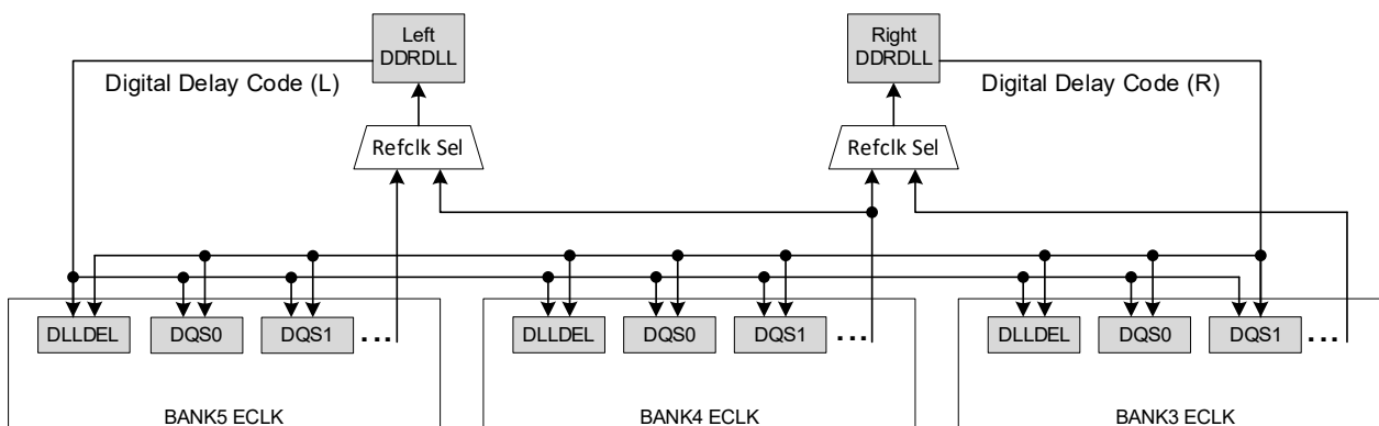
Figure 2.17. DDRDLL Architecture for MachXO5-NX-55T/MachXO5-NX-100T Devices
