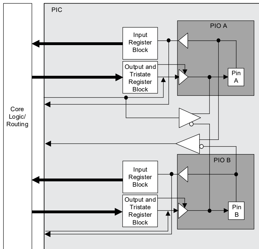
Figure 2.23. Wide Range Programmable (WRIO) I/O Cells
