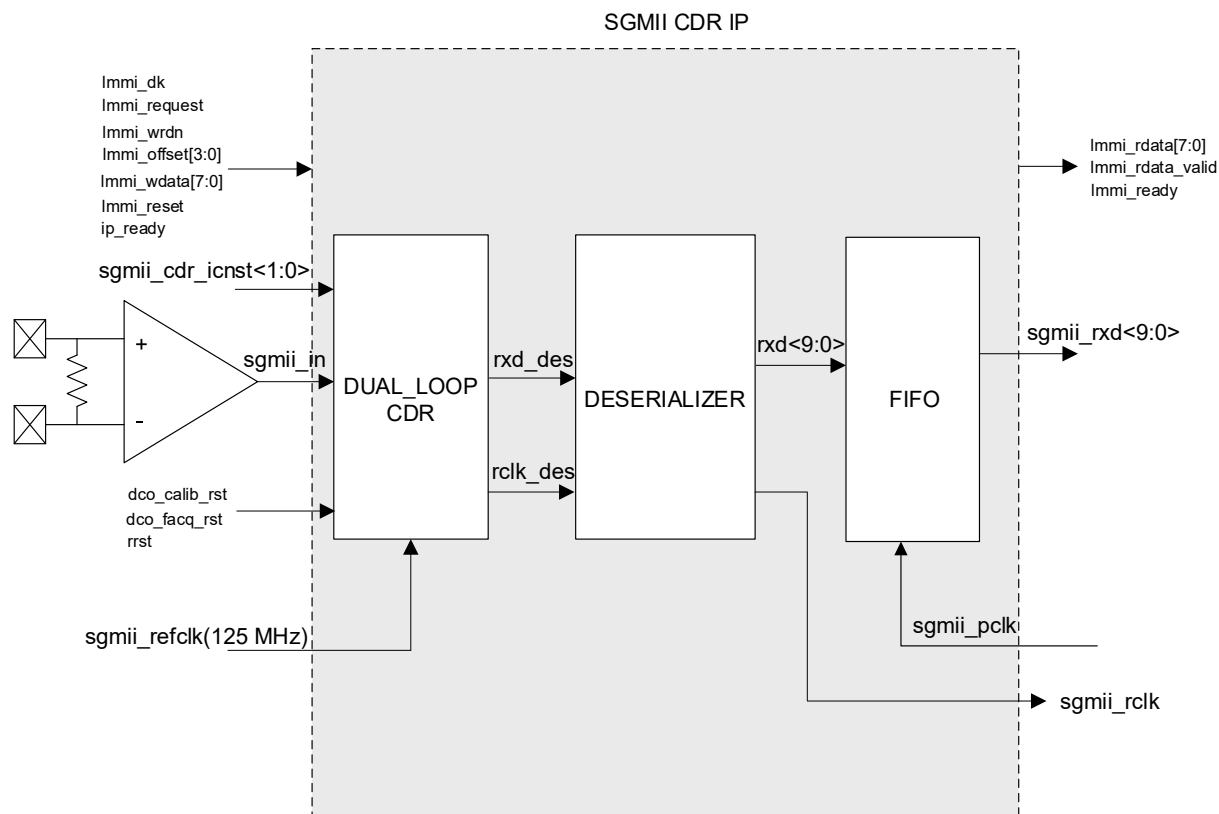
Figure 2.18. SGMII CDR IP
