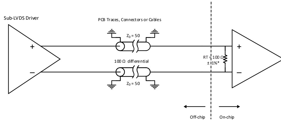
Figure 3.3. SubLVDS Input Interface
