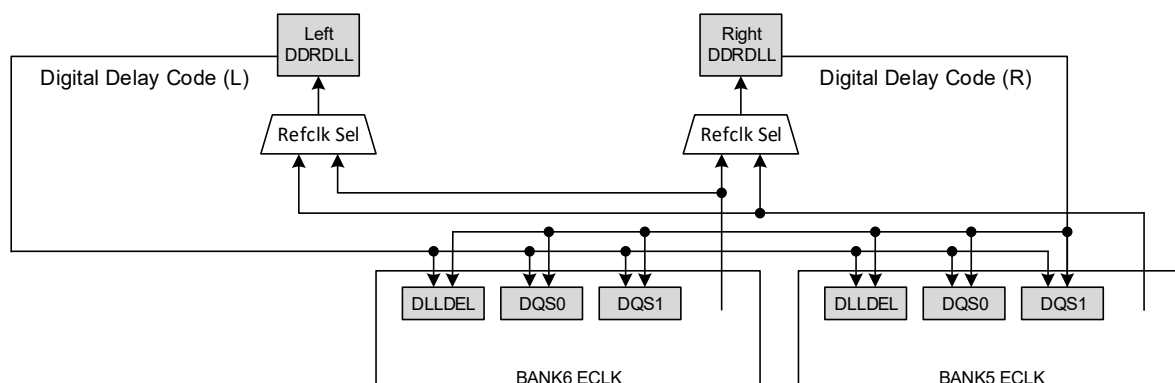
Figure 2.16. DDRDLL Architecture for MachXO5-NX-25 Devices
