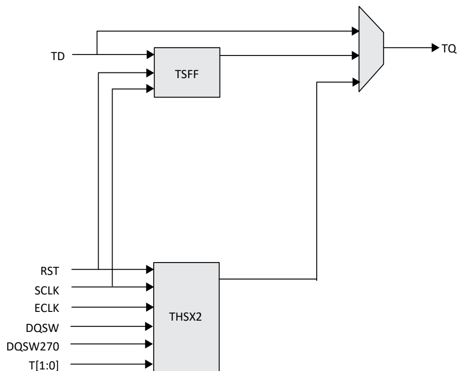
Figure 2.29. Tri-state Register Block on Bottom Side
