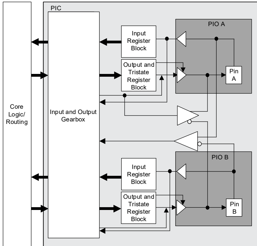
Figure 2.22. Group of Two High Performance Programmable (HPIO) I/O Cells
