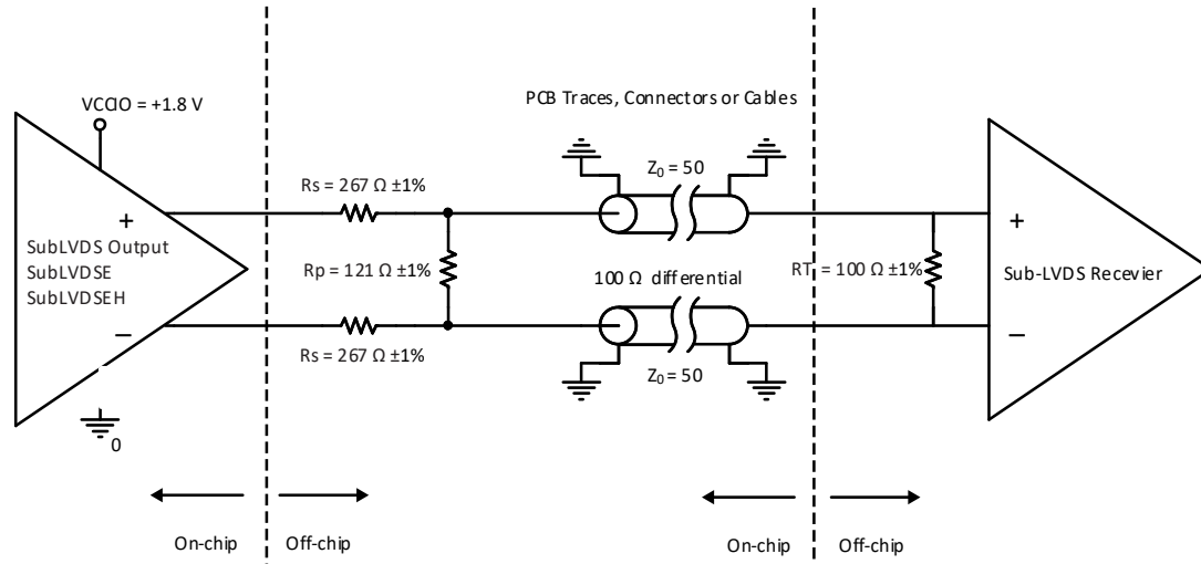
Figure 4.4. SubLVDS Output Interface
