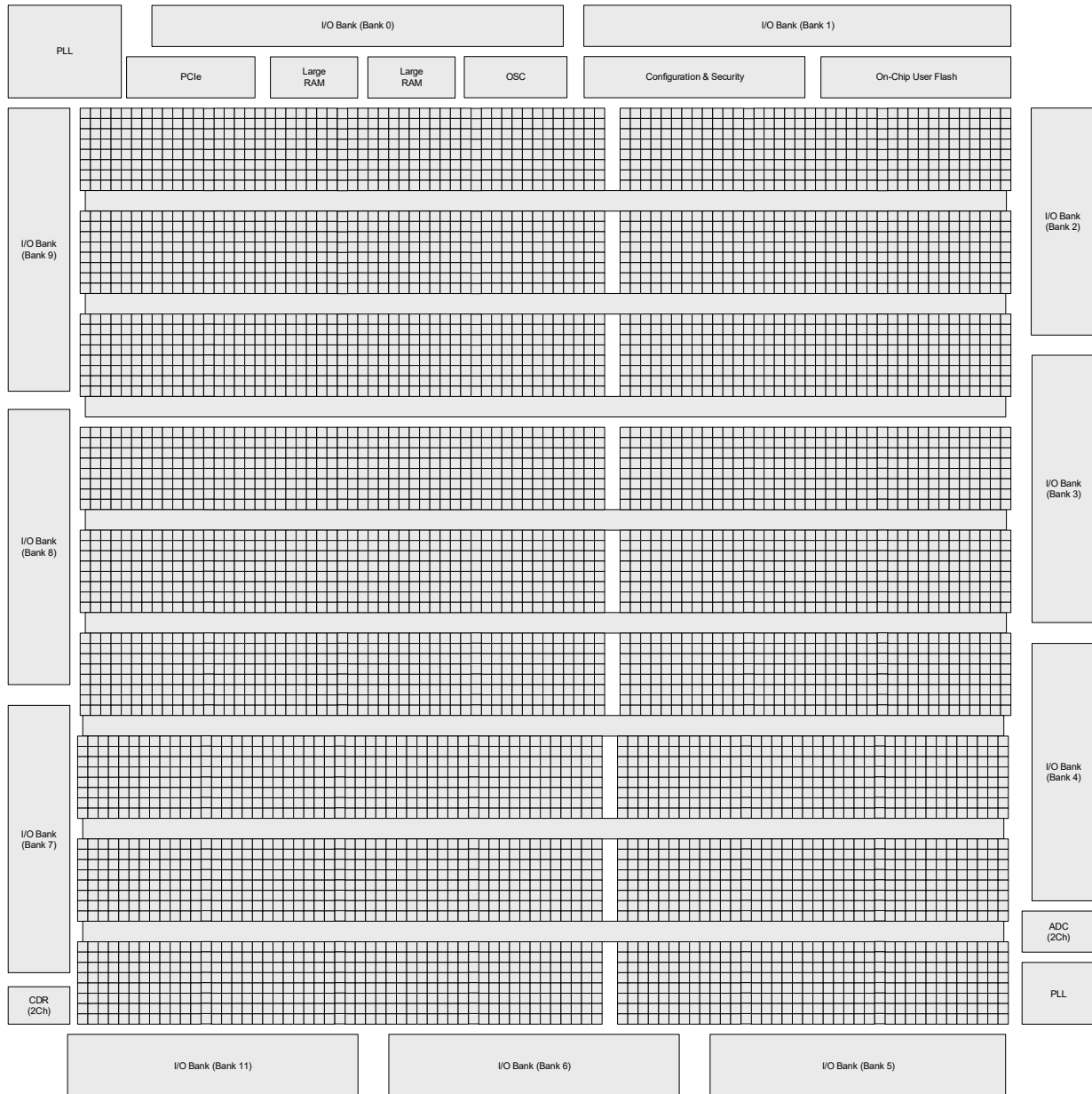
Figure 2.4. Simplified Block Diagram, MachXO5-NX-35/T and MachXO5-NX-65/T Devices (Top Level)
