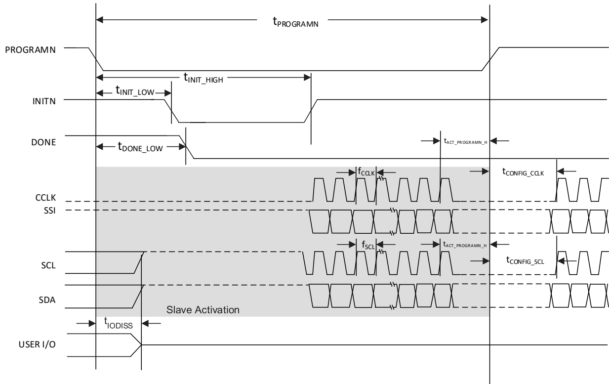
Figure 4.16. Slave SPI/I2C/I3C PROGRAMN Timing
