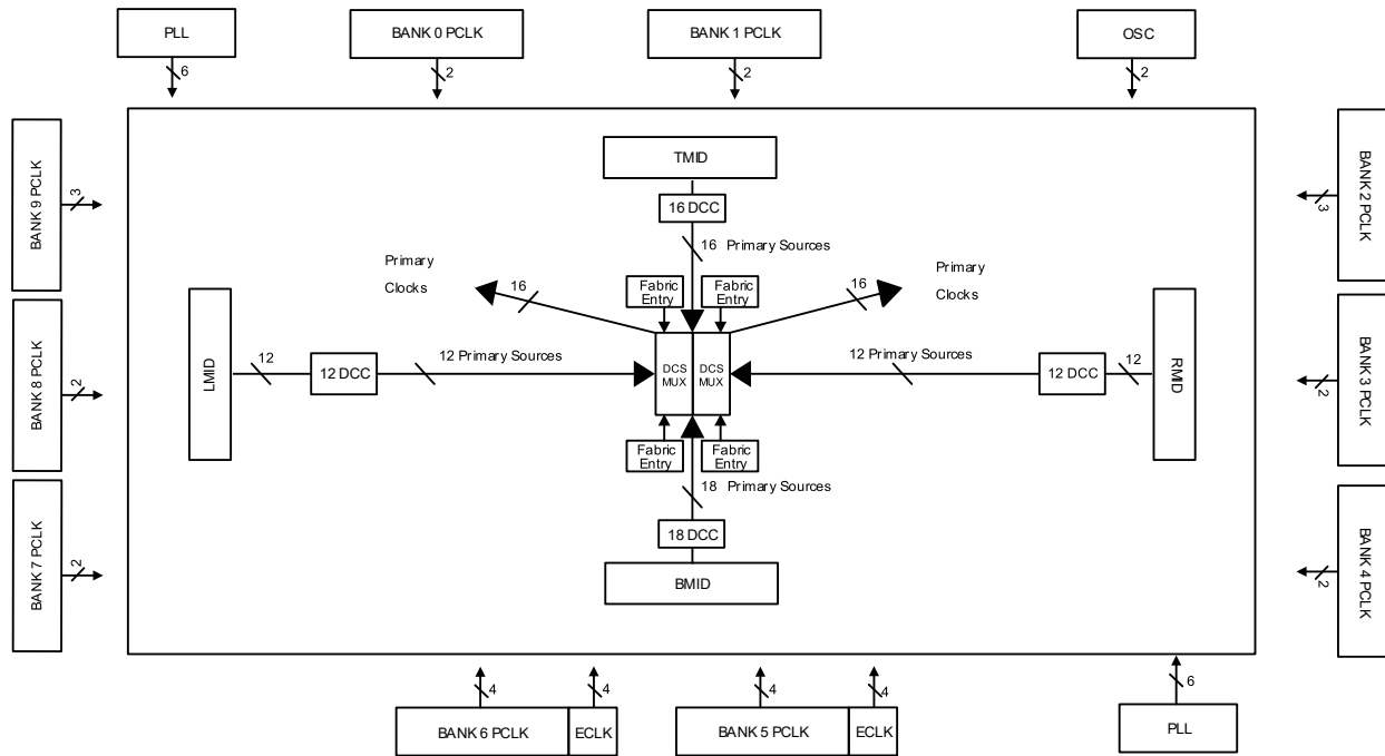
Figure 2.9. Clocking for MachXO5-NX-35/T, MachXO5-NX-65/T, and MachXO5-NX-25 Devices
