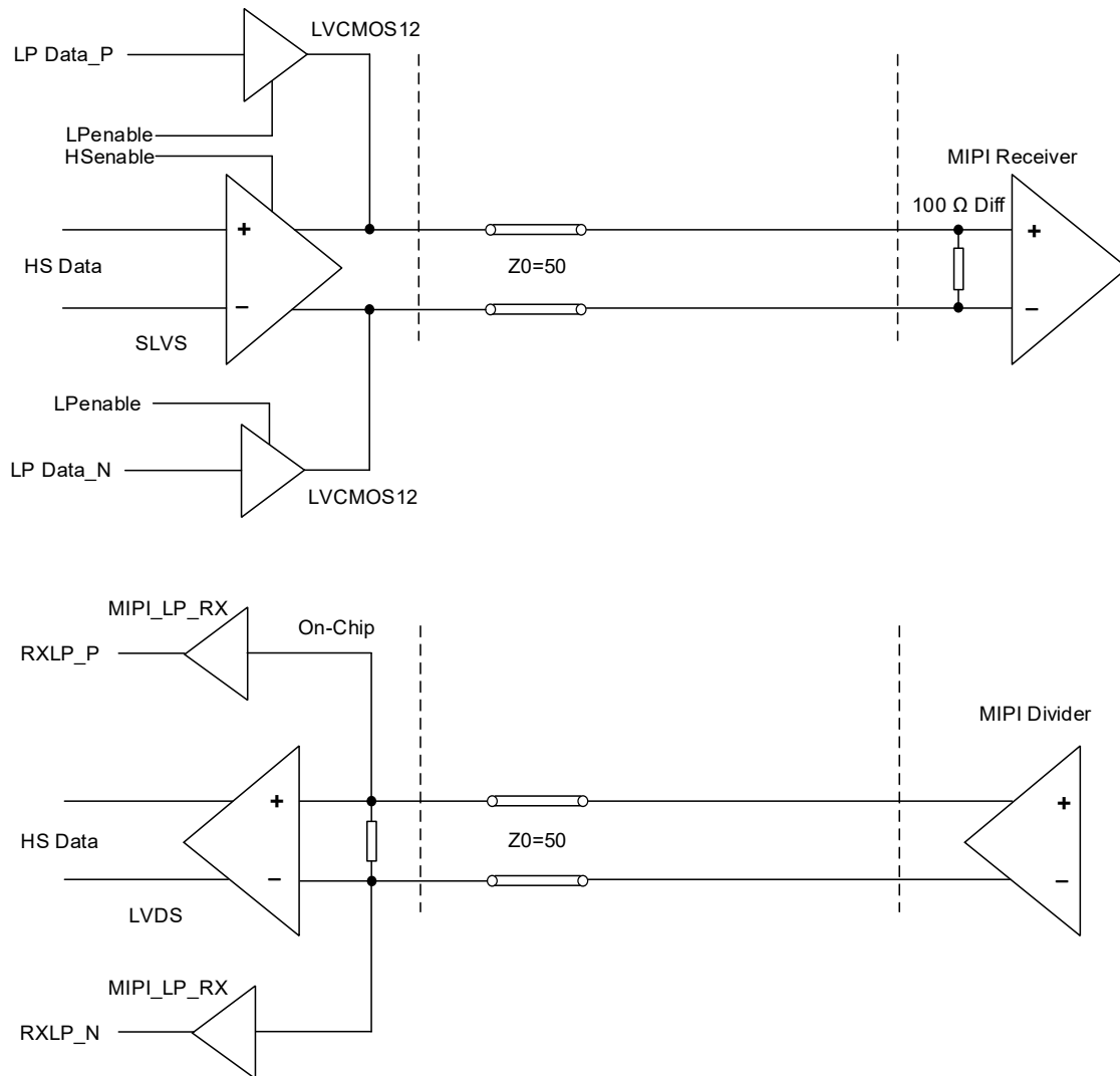
Figure 3.6. MIPI Interface
