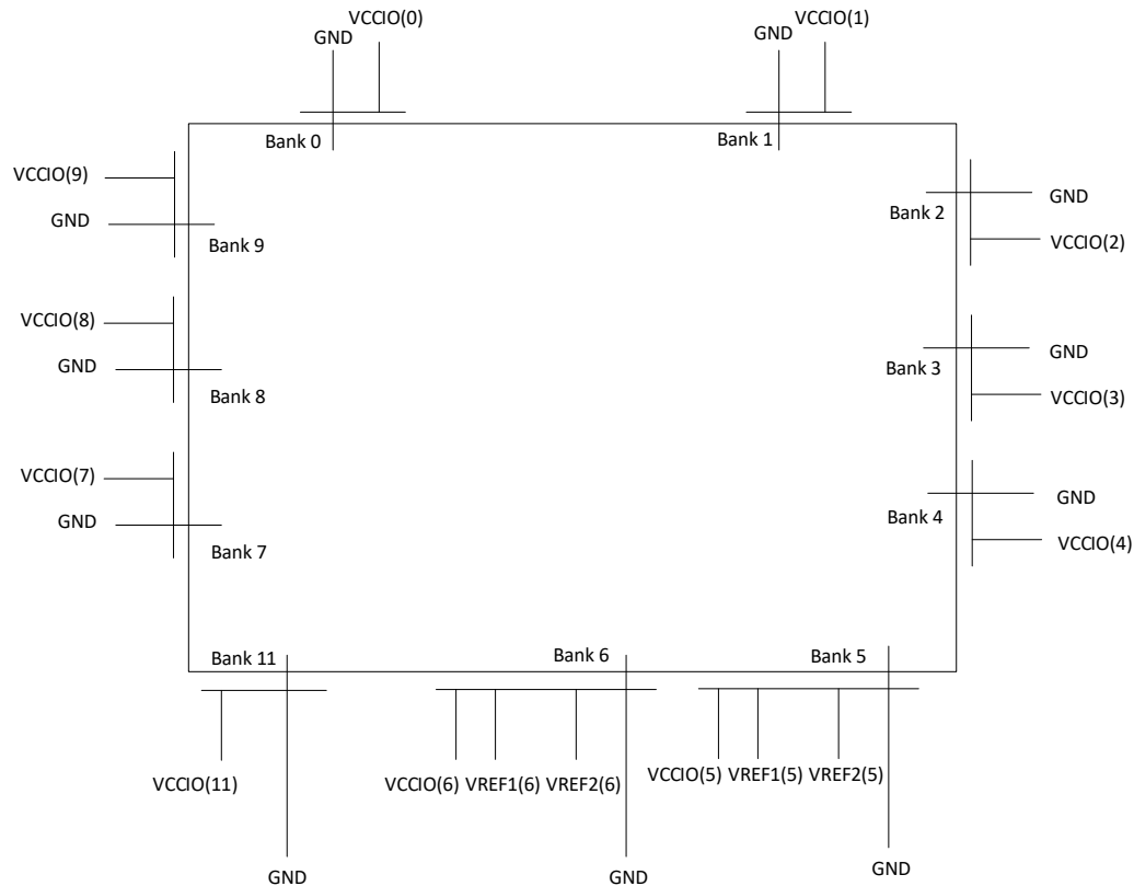
Figure 2.34. sysI/O Banking of MachXO5-NX-35T/MachXO5-NX-65T Devices
