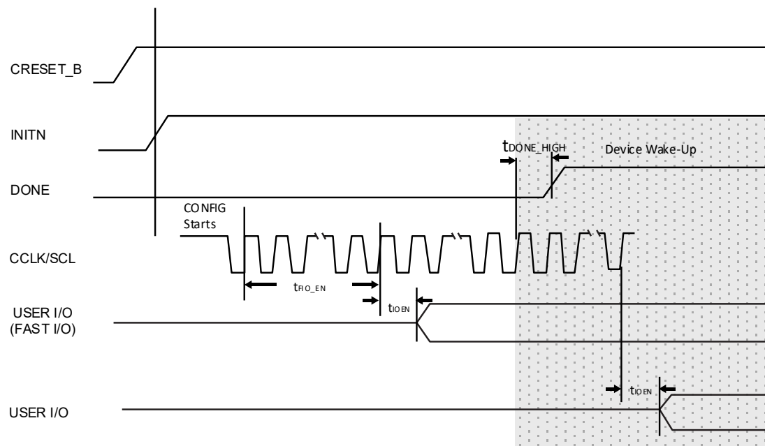
Figure 4.19. Slave SPI/I2C/I3C Wake-Up Timing
