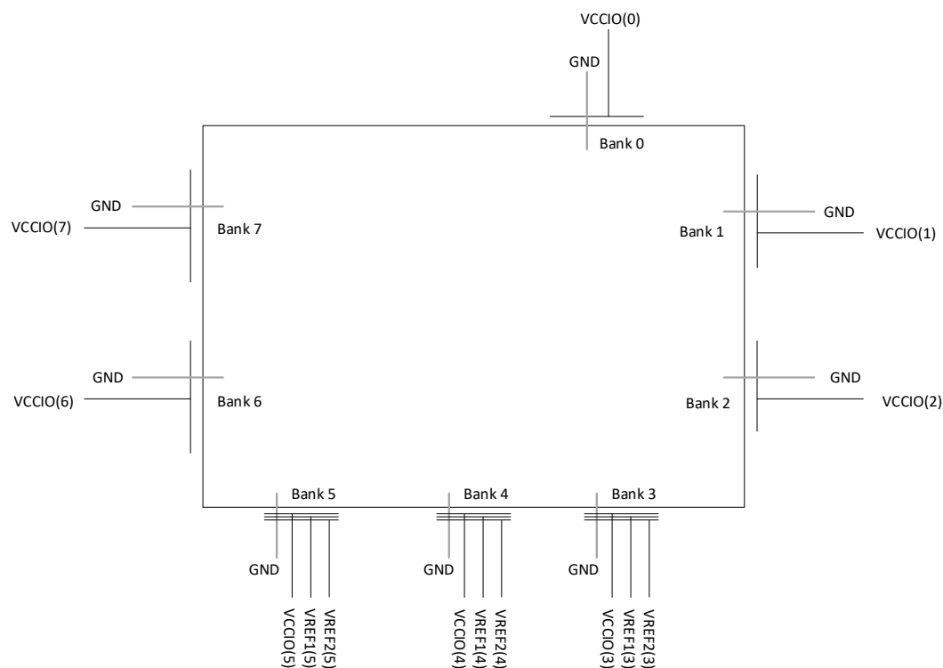
Figure 2.32. sysI/O Banking of MachXO5-NX-25 Devices
