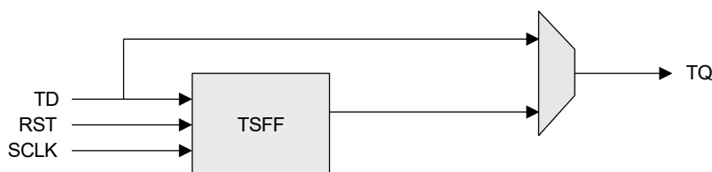
Figure 2.28. Tri-state Register Block on Top, Left, and Right Sides
