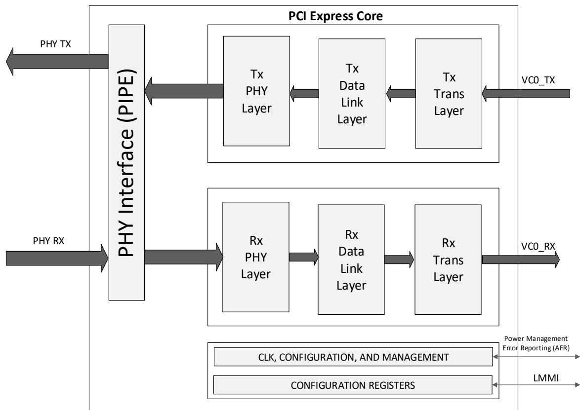
Figure 2.35. PCIe Core
