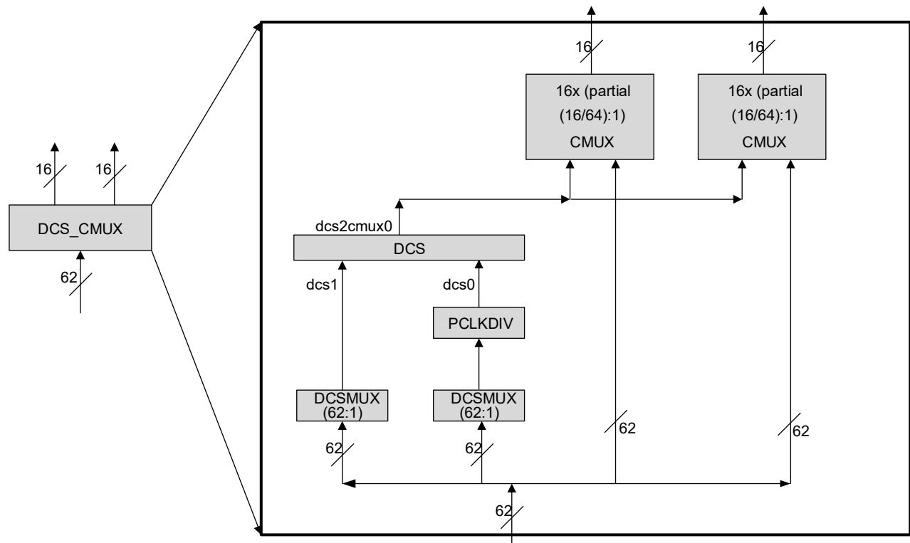
Figure 2.12. DCS_CMUX Diagram for MachXO5-NX-25 Devices
