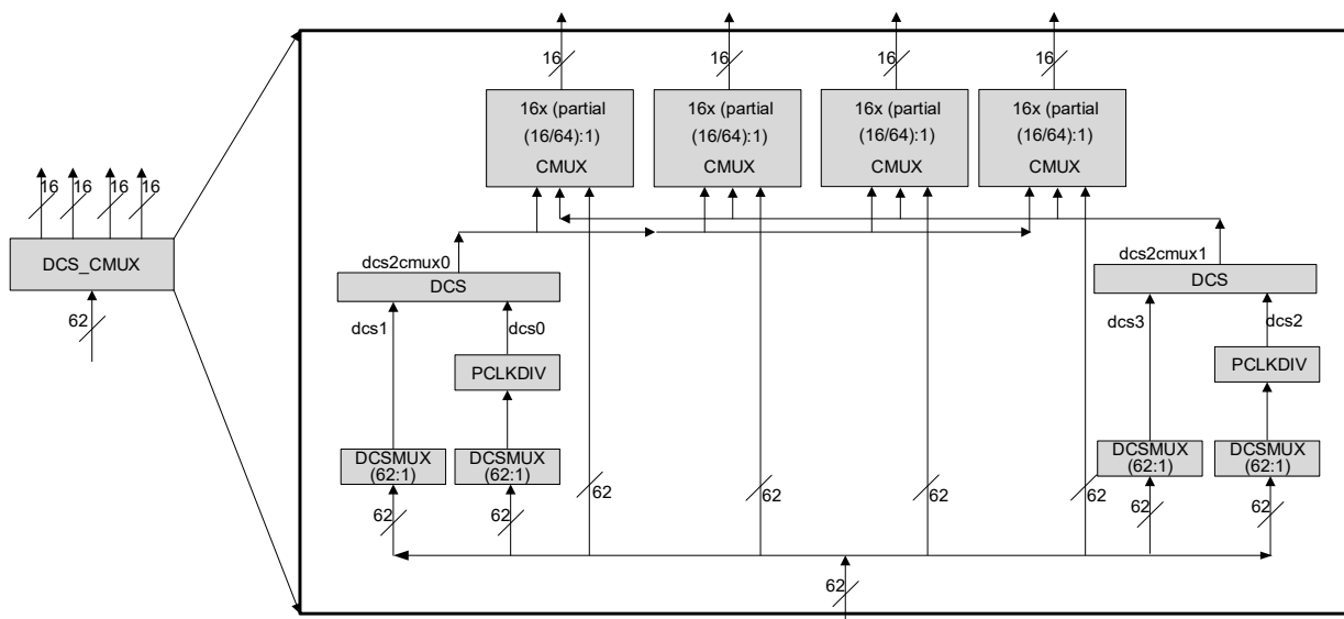
Figure 2.13. DCS_CMUX Diagram for MachXO5-NX-55T/MachXO5-NX-100T Devices
