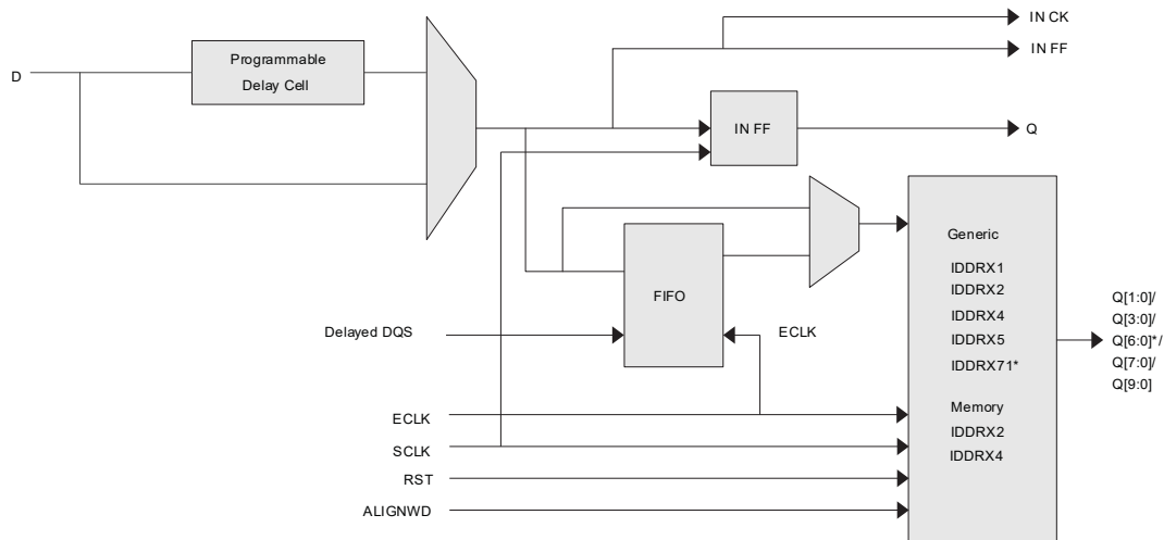
Figure 2.25. Input Register Block for PIO on Bottom Side of the Device
