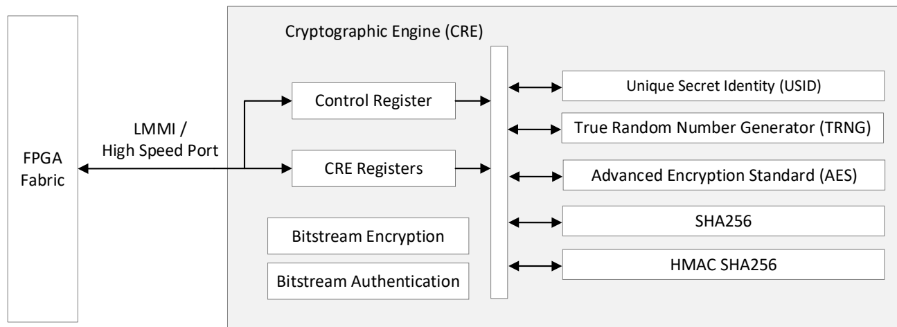
Figure 2.37. Cryptographic Engine Block Diagram
