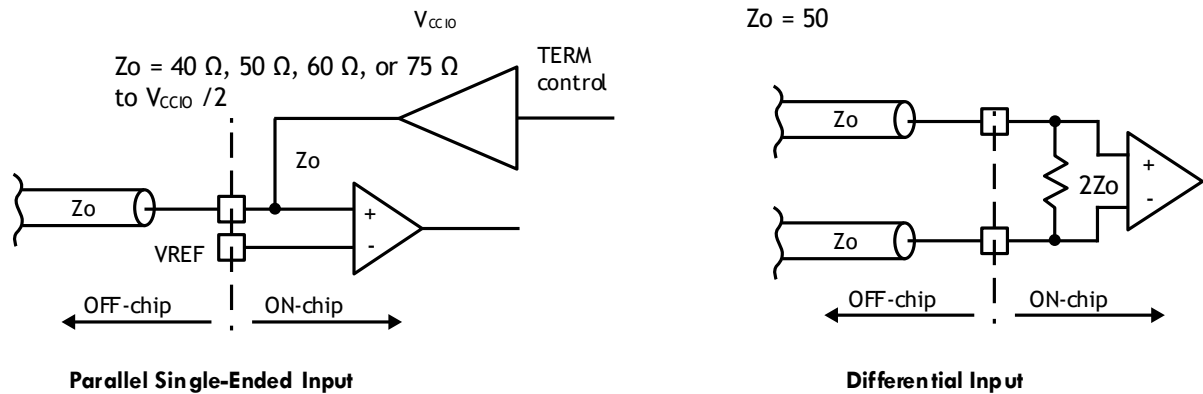
Figure 3.1. On-Chip Termination
