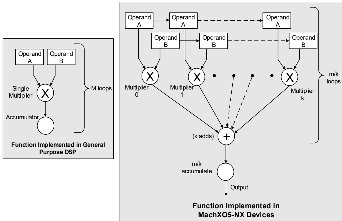
Figure 2.20. Comparison of General DSP and MachXO5-NX Approaches
